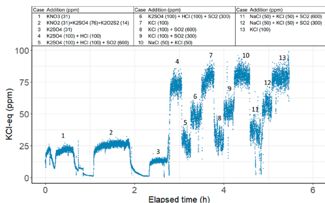
Figure 9. Time-resolved SID data (1 Hz) during different additions of selected alkali salts. During the addition of alkali chlorides, the SID signal corresponds well with the nominal concentration. The lower signal response of sulfates demonstrates the quantification limitation when sampling an unknown gas composition.
