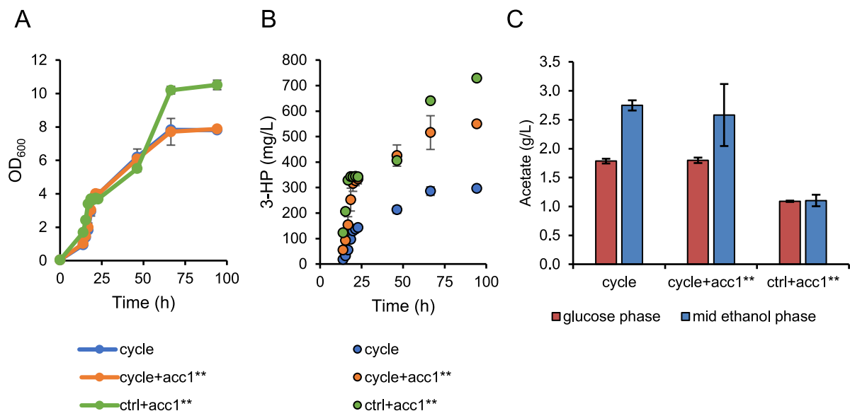
Figure 27. Effect of additional ACC1** overexpression in strains with the phosphoketolase pathway (ctrl) or the GATHCYC (cycle) for additional acetyl-CoA supply on A ) OD 600 profile, B ) 3-HP profile and C ) acetate concentrations. Strains were cultured with biological triplicates in shake flasks using minimal media supplemented with 2% glucose and 100 mg/L uracil. Average values are shown with the standard deviation as errors bars.
