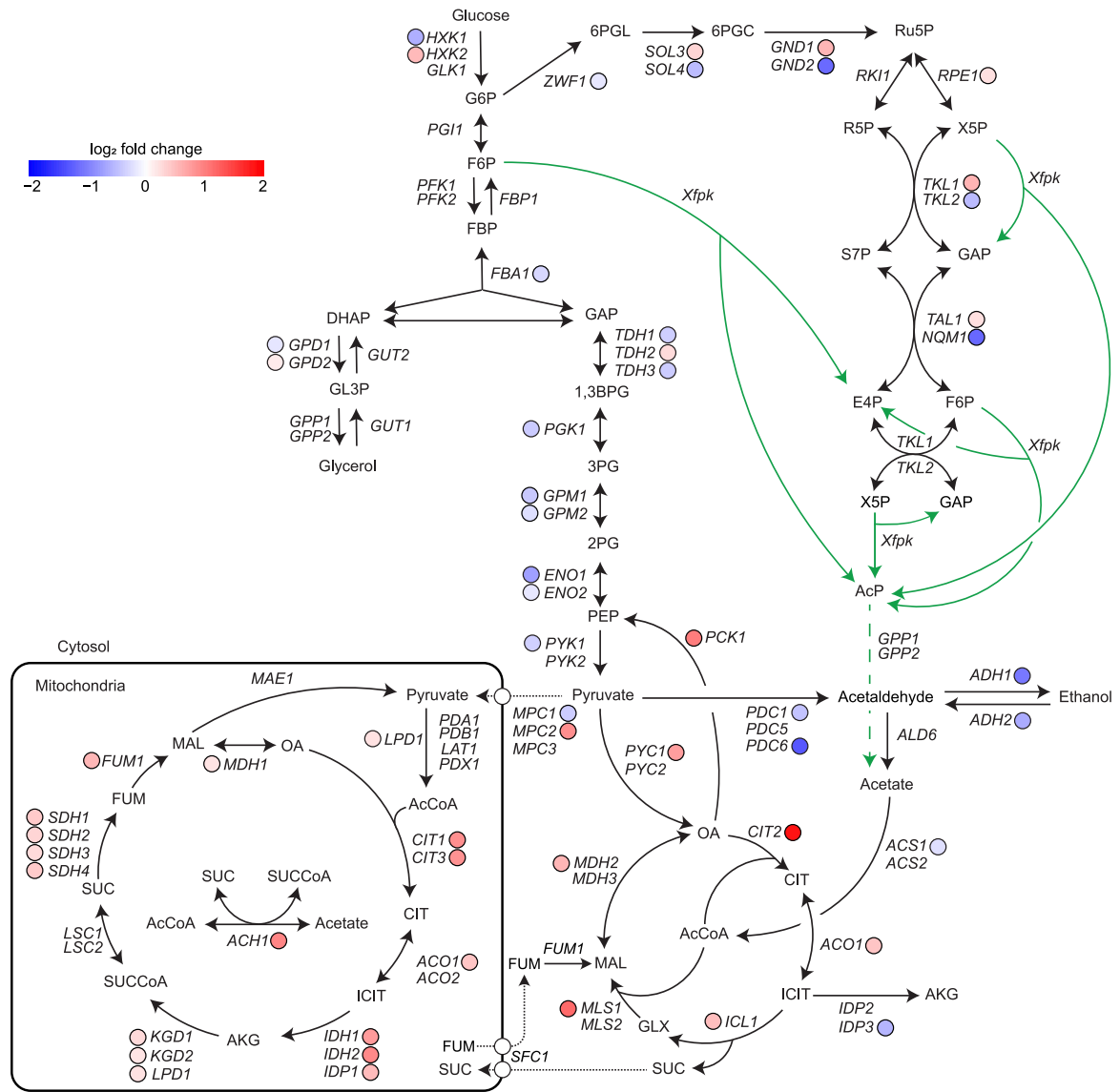
Figure 4. Differentially expressed genes in the central carbon metabolism from phosphoketolase expression during carbon-limited chemostat. The \log_2 -fold change (LFC) values are filtered for adjusted p-value below 0.01 and visualized as intensities of red (up) and blue (down). Full green arrows indicate the introduced phosphoketolase reactions. The dashed green arrow highlights the promiscuous degradation of AcP to acetate by Gpp1 and Gpp2. Figure adapted from Paper I [88].
