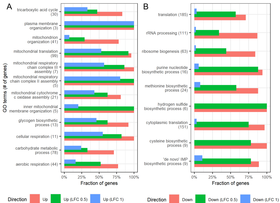
Figure 12. GO-terms involved in biological processes that are enriched for A) upregulated or B) downregulated genes from STB5 overexpression during batch growth on glucose at pH 5. Data summarized from the consensus heatmap generated with the Piano R-package by filtering the median adjusted p-value below 0.1 for non-directional enrichment and below 0.05 for the distinct up- or downregulated enrichment. The fraction of up- or downregulated genes is shown without filtering (red) and absolute LFC > 0.5 (green) or absolute LFC > 1 (blue) together with an adjusted p-value below 0.01.
