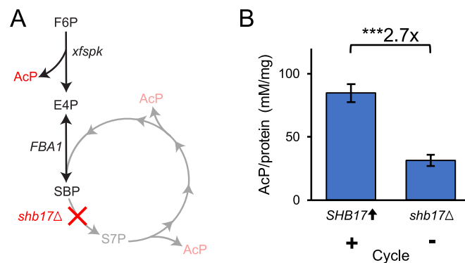
Figure 18. In vitro evaluation of AcP production on crude cell-free extracts from S. cerevisiae containing the genotype for the GATHCYC. A) Deleting SHB17 stops utilization of the full cycle (faded) and should result in three times less AcP from F6P compared to SHB17 overexpression. B) In vitro AcP formation from GATHCYC strains with SHB17 overexpression or SHB17 deletion. Statistical significance was evaluated with a two-sided Student’s t-test with unequal variance (***p < 0.001). Figure adapted from Paper III [118].
