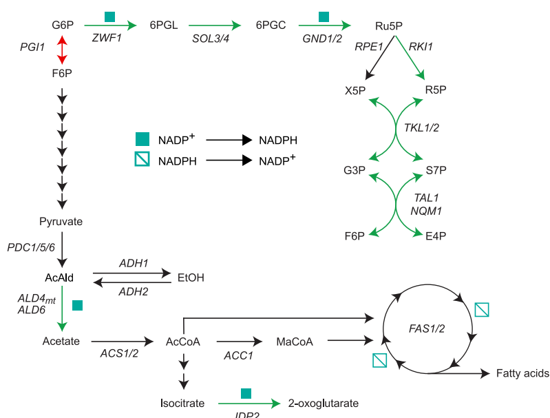
Figure 7. Overview of targets of Stb5 in central carbon metabolism. Green and red arrows indicate genes that are activated or repressed, respectively, by Stb5. Abbreviations: AcAld, acetaldehyde; MaCoA, malonyl-CoA; refer to text for other abbreviations. Figure adapted from Paper II [102].
