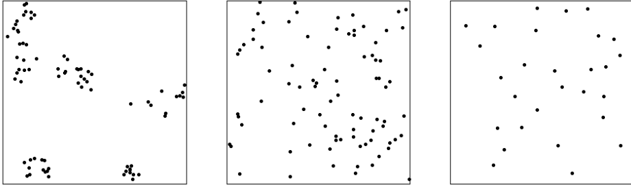
Figure 3.1: The three main types of point patterns: clustered (left), completely spatially random (middle) and regular (right).
