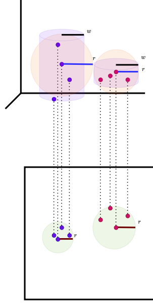
Figure 3.4: Illustration of potential differences in clustering in different dimensions. The projections of the "red" pattern are less clustered in \mathbb{R}^2 but more clustered than the "purple" pattern in \mathbb{R}^3 . The structuring elements for the Ripley's K and cylindrical K functions are also illustrated.
