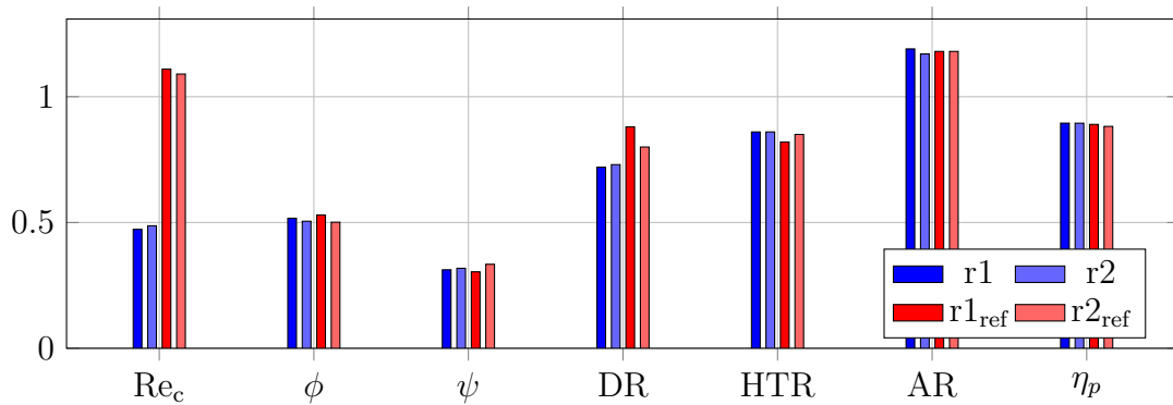
Figure 4.5: Facility compressor parameters in comparison to reference engine parameters. AR – Aspect ratio; HTR - Hub-to-tip ratio; DR – Degree of reaction; Re_c – Chord based Reynolds number; \phi – Flow coefficient; \psi – Stage loading; \eta_p – Polytropic efficiency.
