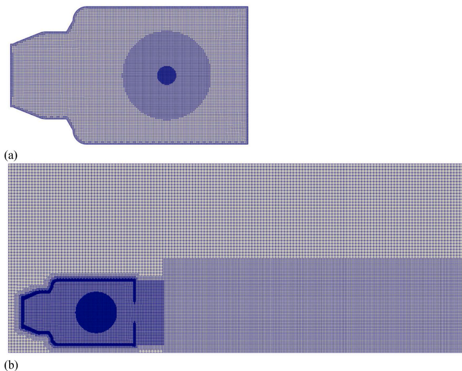
Fig. 4. Two sets of computational meshes. (a) Mesh for closed vessel. (b) Mesh for the vessel and outside domain.
