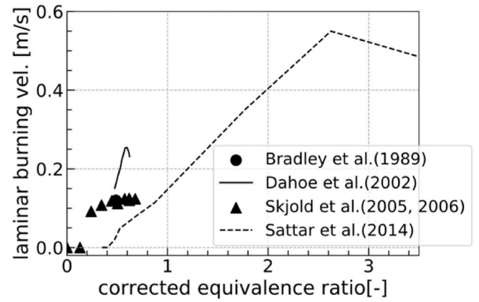
Fig. 3. Comparison of laminar burning velocities for corn starch dust reported by Bradley et al. (1989), Dahoe et al. (2002), Skjold et al. (2005, 2006), and Sattar et al. (2014).
