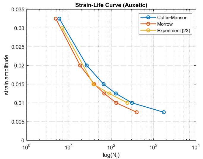
Fig. 11. Numerical and experimental (Tomazincic et al., 2019) strain-life curve for LCF analysis of the auxetic lattice.
