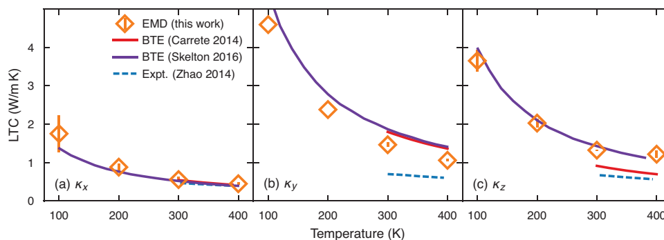
Figure 7. LTC of SnSe calculated using the EMD method (orange diamonds) based on a sixth-order FCP together with BTE calculations by Carrete et al. [66] (red solid line) and Skelton et al. [66] (purple solid line) as well as experimental measurements by Zhao et al. [68] (blue dashed line).
