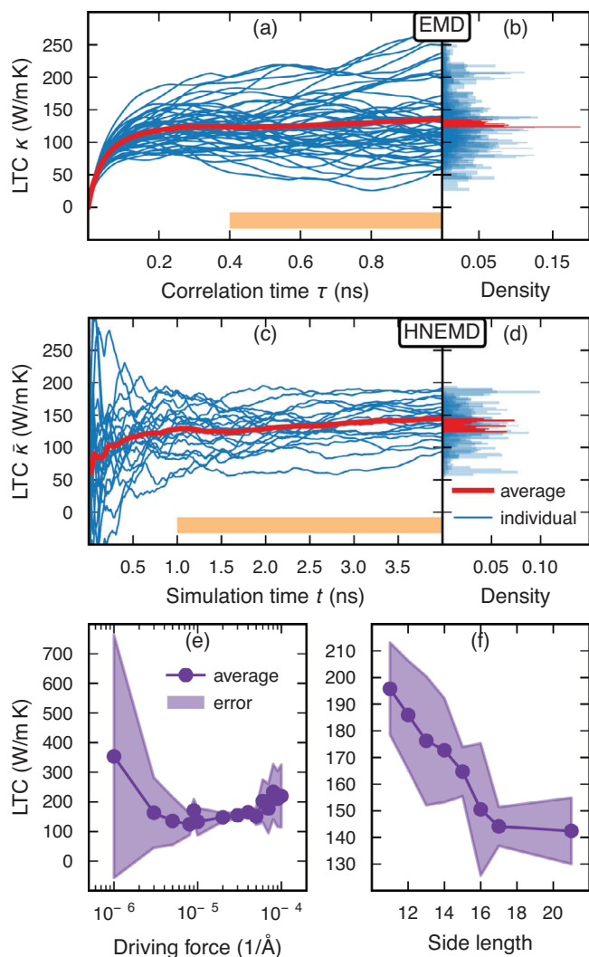
Figure 4. LTC of ml-MoS 2 at 300 K from a,b) EMD simulations according to Equation 3 and c,d) HNEMD simulations according to Equation 8 with F_e^x = 4 \times 10^{-5} \text{ \AA}^{-1} . All simulations were based on the sixth-order model and used a 16 \times 16 \times 1 supercell. a,c) The results from independent runs are shown by thin blue lines while the average is indicated by red thick lines. b,d) The histograms were generated by averaging the data after equilibration as indicated by the orange bars. Convergence of LTC from HNEMD simulations with e) driving force for a 15 \times 15 \times 1 supercell and f) system size (side length in units of the ml-MoS 2 lattice constant) for F_e^x = 4 \times 10^{-5} \text{ \AA}^{-1} based on the fourth-order model.
