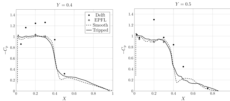
Figure 5. Distribution of the pressure coefficient at different sections of the Twist11 foil.
