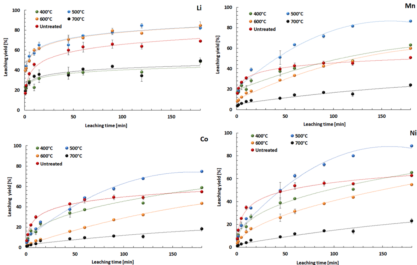
Fig. 1. Leaching yield of Li, Mn, Co and Ni from incinerated samples after 1 h of incineration. Leaching media: 2 M H 2 SO 4 at 25 °C after 180 min. The sequence of the plots: Li; Mn; Co and Ni.
