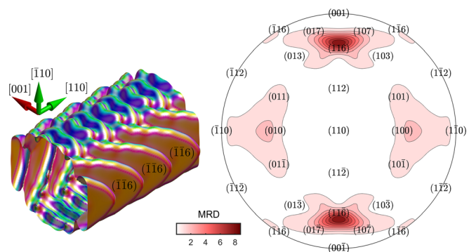
FIG. 6. Nanorod morphology obtained for M/|\bar{R}| = 0.01 . The upper pole figure is superimposed with the lower for this morphology.
