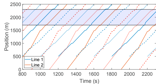
Fig. 5. Trajectory of every bus in the network. Different line styles are used to distinguish individual buses. Trajectories of Line 1 are shifted so positions match in the common line section.
