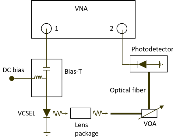
Figure 3.6: Measurement setup for small-signal modulation response.
