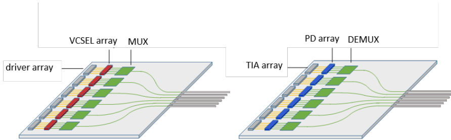
Figure 2.2: Left: SiP transmitter with flip-chip mounted multi-wavelength VCSEL arrays, multi-channel drivers and integrated MUXs. Right: SiP receiver with flip-chip mounted PD arrays, multi-channel TIAs and integrated DEMUXs.
