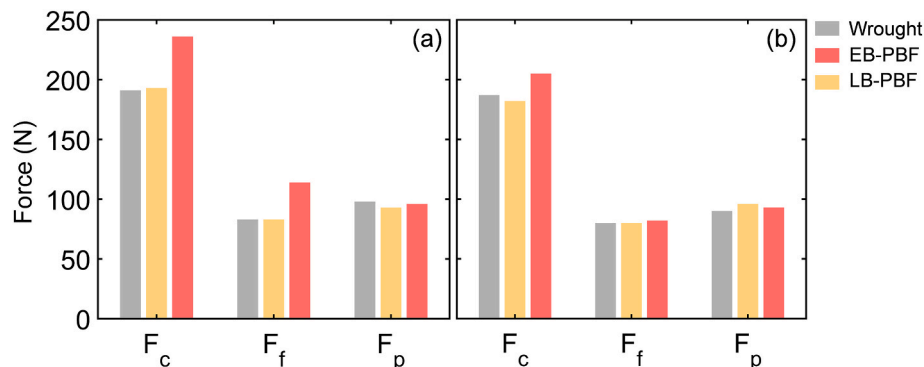
Fig. 12. Cutting (F c ), feed (F f ) and passive (F p ) forces measured when machining wrought, EB-PBF and LB-PBF materials in as-received and as-built conditions (a), and after solutionising and aging treatment (b). The results represent the measurements in the beginning of the tests (10 s) using a fresh tool.
