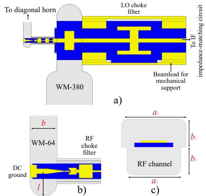
Fig. 4. EM model for the 3.5-THz, \times 6 -harmonic Schottky diode mixer. (a) Full 3D-EM model of the integrated planar Schottky diode realized on a 2- \mu\text{m} -thick GaAs substrate, which is suspended on an E-plane split block using beam leads. (b) RF chain consisting of a WM-64 waveguide, dc grounded RF E-plane probe, Schottky diode contact, and RF choke filter. (c) Cross section image of the RF filter channel.
