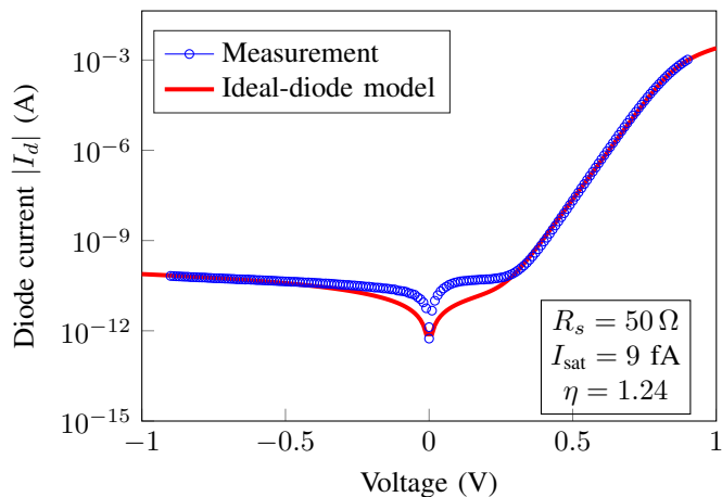
Fig. 13. Diode current-voltage characteristic. Comparison of the diode model and on-wafer dc-measurements of a fabricated \times 6 -harmonic Schottky diode integrated mixer circuit with a Schottky contact area of 0.11 \mu\text{m}^2 . Extracted diode parameters are as shown. The measurements were performed with Kelvin probes at room temperature (dark condition). The applied dc-voltage was swept from -0.9 to +0.9 V as the maximum current was limited to 1 mA.
