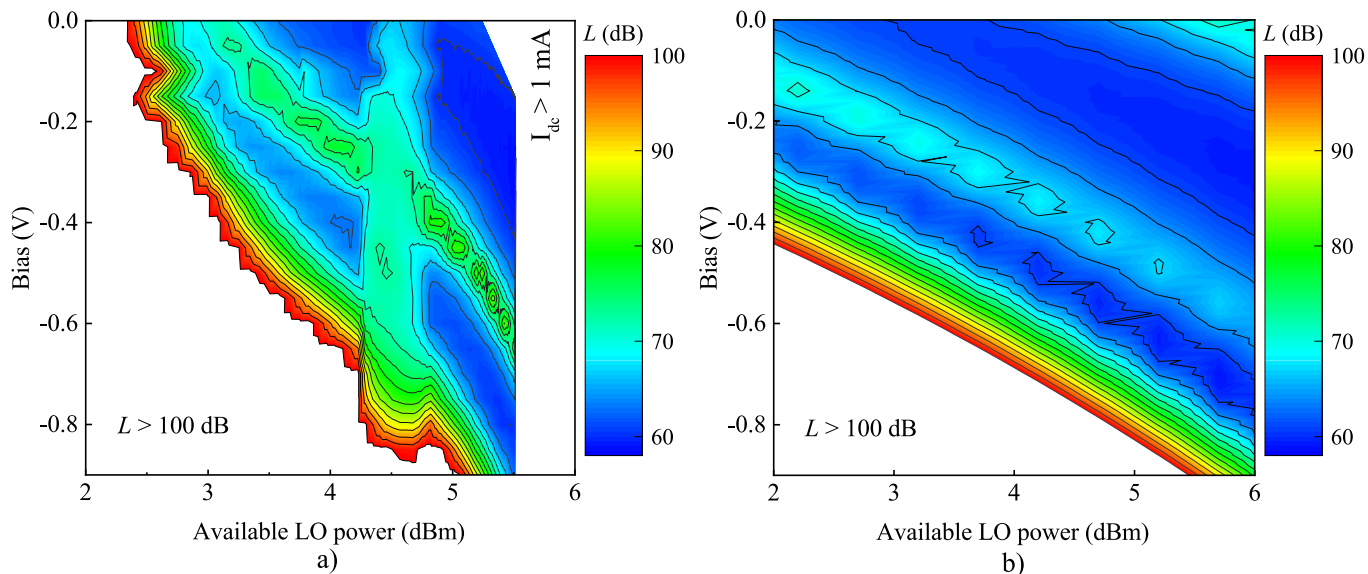
Fig. 14. Conversion loss as a function of LO power and bias. (a) Measurement: Conversion loss measured at an IF of 200 MHz, an RF of 3.443 THz, and for an LO signal at 573.3 GHz. The measured RF power at the mixer interface was about -3 dBm and the available LO power was about 5.6 dBm at 573 GHz. At low LO powers, the measurement is affected by the noise floor of the system, while at higher powers it is limited by the maximum available LO power. (b) Simulation: Harmonic-balance simulation with an ideal-diode model assigned with parameters extracted from the dc measurements. The contour step is 3 dB.
