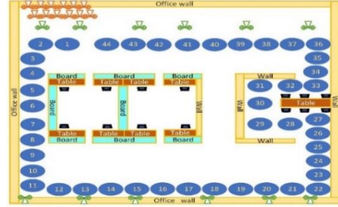
Fig. 3. Indoor layout for measurement. Green and orange antennas represent placement of distributed- and co-located antennas, respectively. Whole area is enclosed by walls and there are boards, tables, chairs and a conference room. The numbered blue circles are measurement positions.
