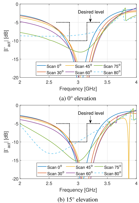
FIGURE 5. Simulated |\Gamma_{act}| of unitcell of antenna element in infinite array environment at various azimuth directions.
