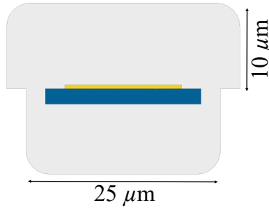
Figure 3.7: Cross section of the RF channel 3D-EM model showing the 2-μm-thick GaAs membrane and 0.5-μm-thick gold striplines defining the stepped-impedance filter.
