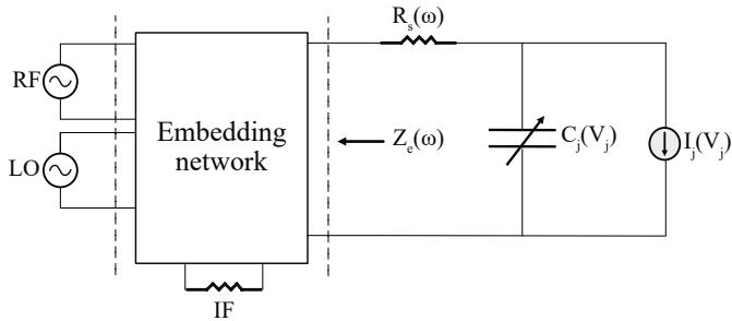
Figure 3.3: Mixer embedding network. The series resistance of the diode and the embedding impedance are analysed in frequency domain. The non-linear junction capacitance and conductance are represented in time domain.
