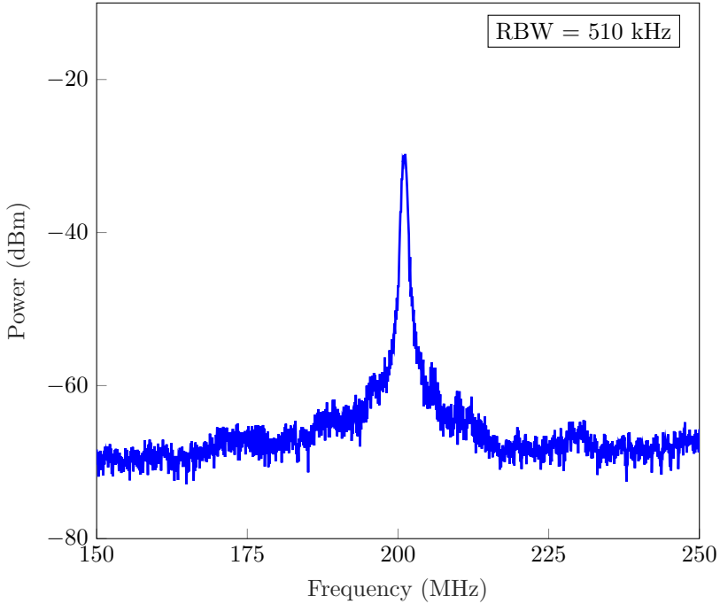
Figure 4.11: Down-converted IF signal at 200 MHz from the harmonic mixer recorded with a resolution bandwidth of 510 kHz and a video bandwidth of 10 kHz.
