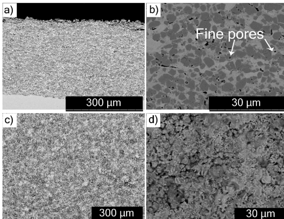
Fig. 2 – SEM analysis of HVOF sprayed \text{Cr}_3\text{C}_2 -NiCr coating: (a & b) cross-section (c & d) top surface.
