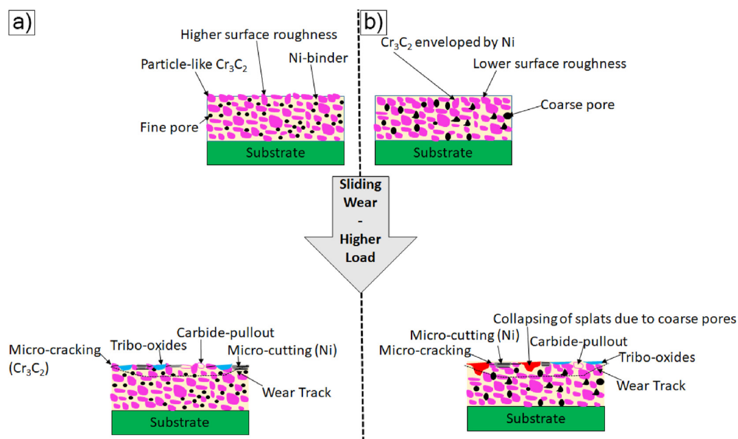
Fig. 19 – Illustration of sliding wear behavior and degradation mechanisms of \text{Cr}_3\text{C}_2 -NiCr coatings deposited by a) HVAF, and b) HVOF.
