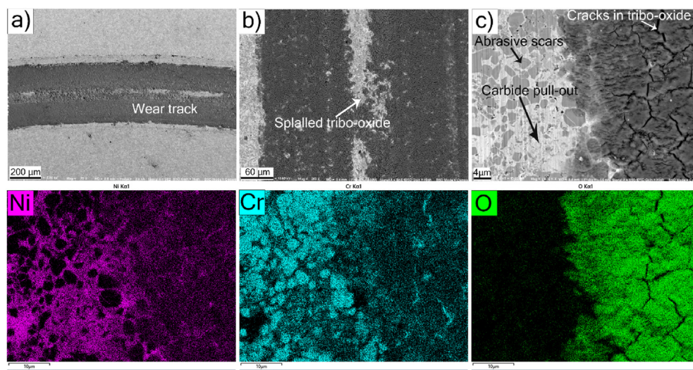
Fig. 12 – SEM/EDS analysis of the worn HVAF coating after ball-on-disc testing at a load of 5 N a) micrograph of wear track b) micrograph showing splalled tribo-oxide layer c) micrograph showing carbide pullout, cracks in tribo-oxide layer along with the corresponding elemental maps.
