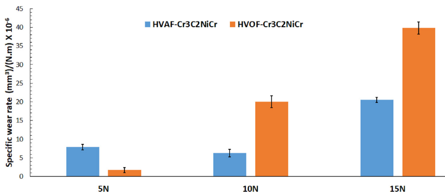
Fig. 9 – Specific wear rates of the HVAF and HVOF sprayed \text{Cr}_3\text{C}_2\text{-NiCr} coatings at different normal loads.
