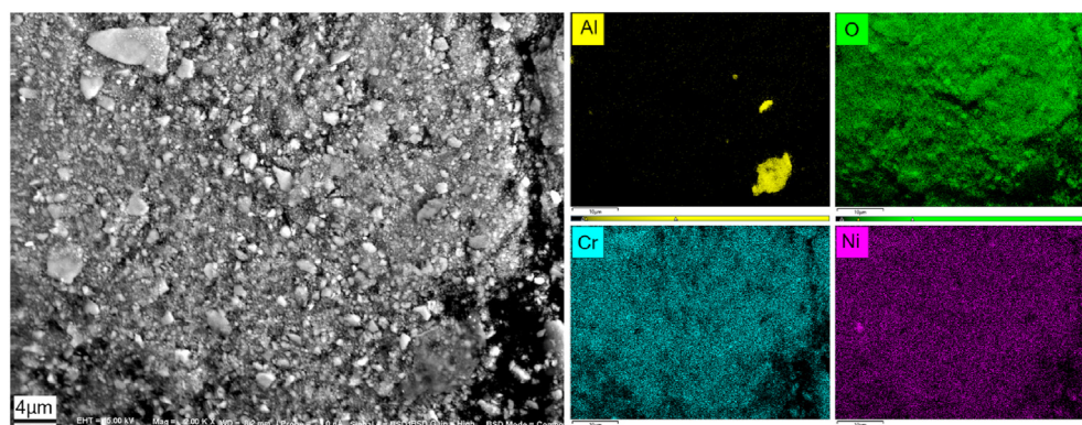
Fig. 13 – SEM/EDS analysis of wear debris generated from the HVAF coating at 5 N normal load.
