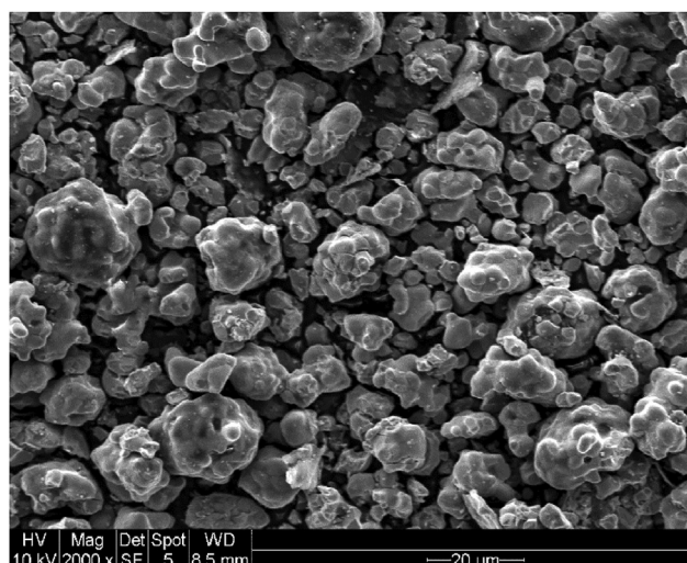
Fig. 1 – SEM analysis of the Cr 3 C 2 -NiCr feedstock.
