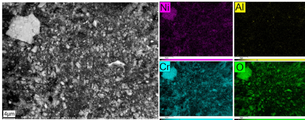
Fig. 18 – SEM/EDS analysis of the wear debris of the HVAF coating subjected to 15 N normal load.
