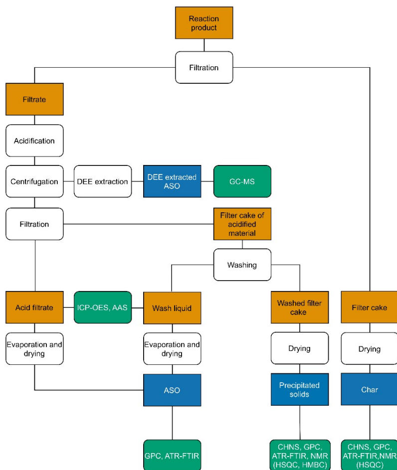
Figure 9: Flowchart of the fractionation of the reaction product and ensuing analyses.
