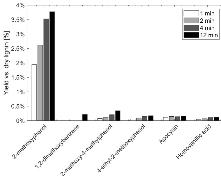
Figure 25: The most prevalent compounds identified by GC-MS in the time series run at 290 °C with IPA/dry lignin 2.7 (w/w), and their respective yield vs. lignin added (determined semi-quantitatively).
