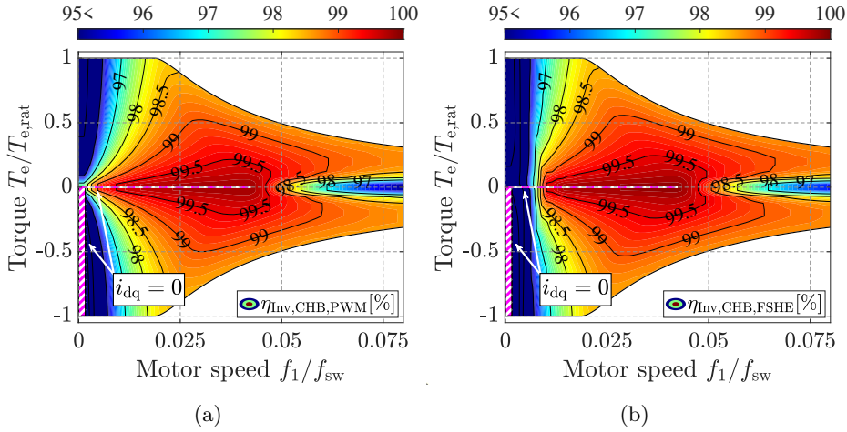
Figure 4.12: Simulated inverter efficiency \eta_{Inv} for the entire drivetrain operating range for (a) multilevel PWM and (b) FSHE.
