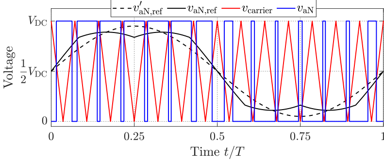
Figure 2.3: Naturally sampled voltage synthesis of the pole voltage v'_{aN,ref} using PWM with optimal zero sequence injection, resulting in v_{aN,ref} , and m_f = 14 .
