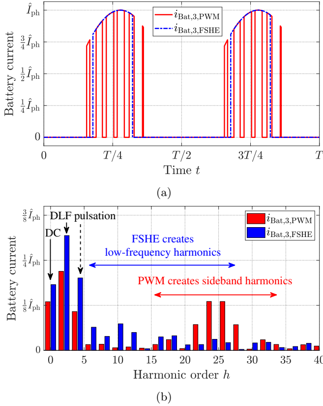
Figure 4.3: (a) Drained battery currents for one battery pack of a seven-level CHB inverter when using multilevel PWM and FSHE for a modulation index M = 0.9 and a carrier ratio of m_f = 40 (PWM). (b) Corresponding harmonic components.
