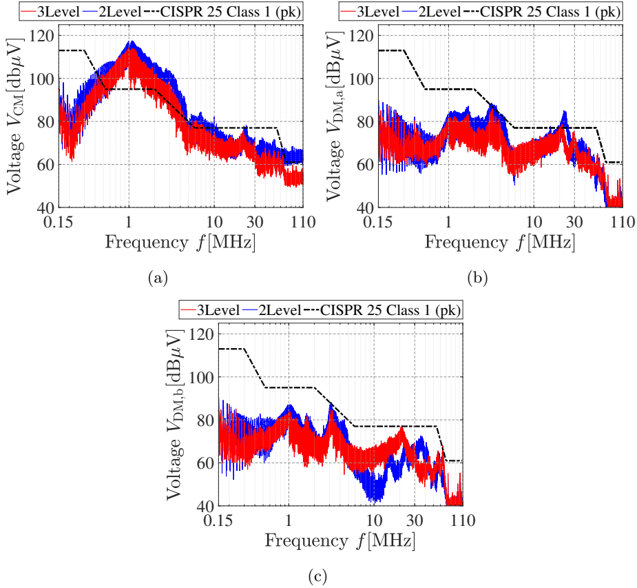
Figure 6.10: Measured (a) CM and (b) phase-DM at positive ( V_{DM,a} ) and (c) neutral DC-link rail ( V_{DM,b} ), when operating the three-level NPC inverter with two-level and three-level modulation.
