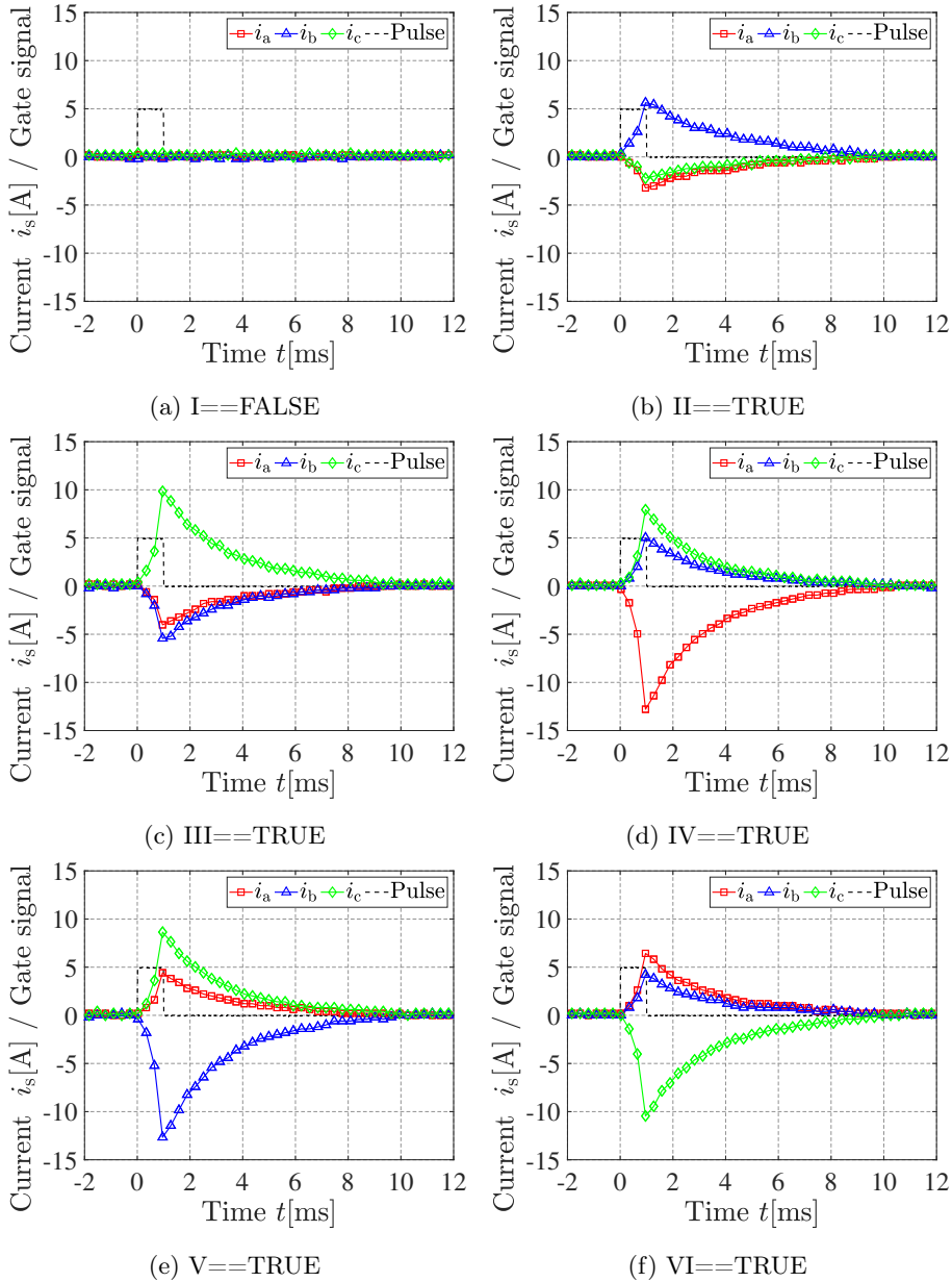
Figure 5.16: Measured pulse responses for a localization of an open circuit fault at S_{a1} for the NPC inverter. Cases from Table 5.1: (a) I==FALSE ; (b) II==TRUE ; (c) III==TRUE ; (d) IV==TRUE ; (e) V==TRUE and (f) VI==TRUE .
