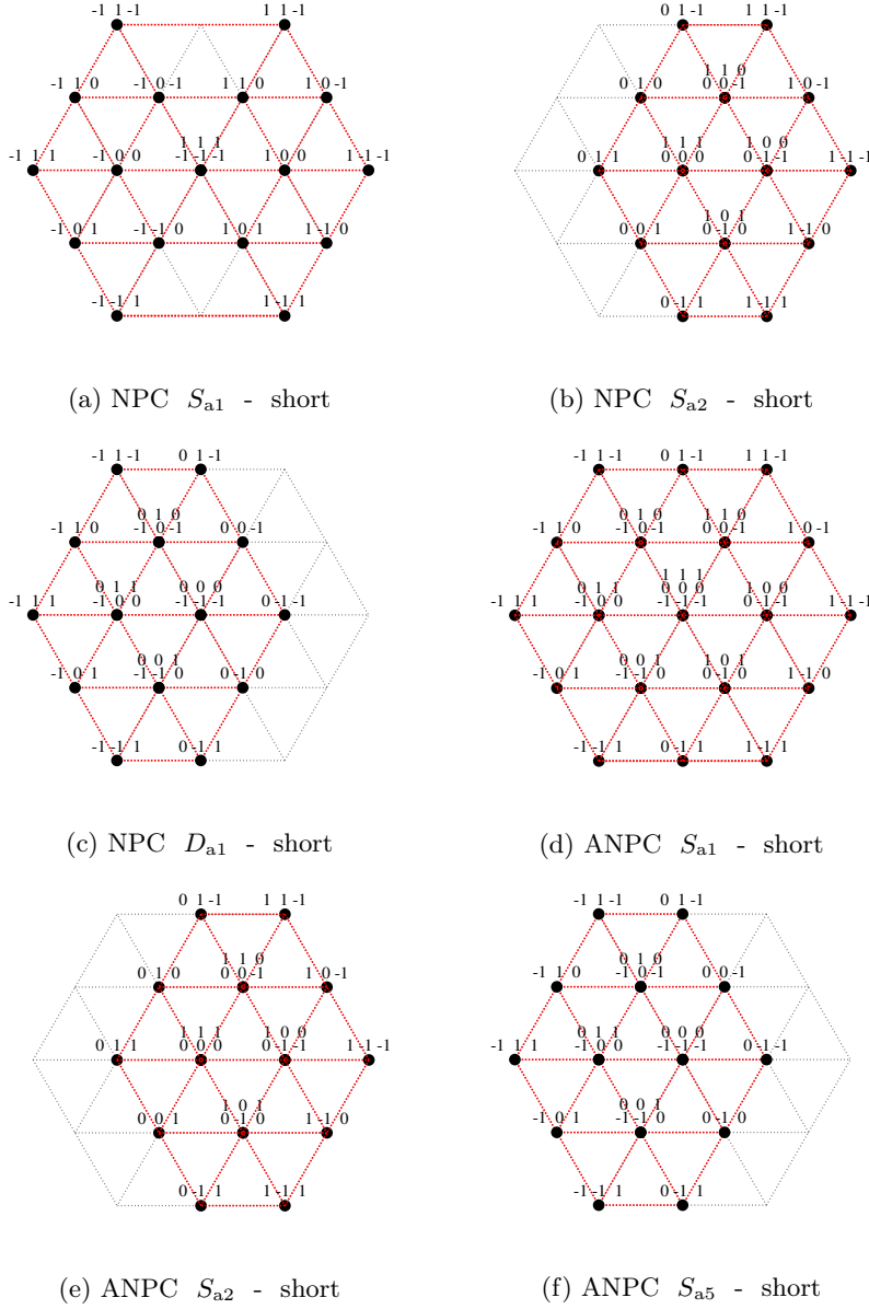
Figure 5.4: Space vector diagram for the corresponding short circuit fault of the three-level NPC and ANPC inverter. Short circuit fault location: (a) NPC S_{a1} –short; (b) NPC S_{a2} –short; (c) NPC D_{a1} –short; (d) ANPC S_{a1} –short; (e) ANPC S_{a2} –short and (f) ANPC S_{a5} –short.
