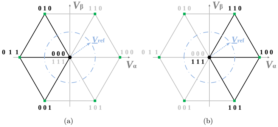
Figure 2.6: Adaption of the space vector diagram in the \alpha\beta -plane in case of a permanent (a) open circuit fault and (b) short circuit fault of the high side switch of phase a.
