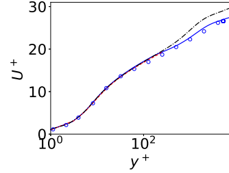
Figure 4: Channel flow. NZ S-DES compared with standard DES . —: DES solver in NZ S-DES; - - -: RANS solver in NZ S-DES; - - - -: Standard DES; \circ : Reichardt's law, U^+ = \frac{1}{\kappa} \ln(1 - 0.4y^+) + 7.8 [1 - \exp(-y^+/11) - (y^+/11) \exp(-y^+/3)] .
