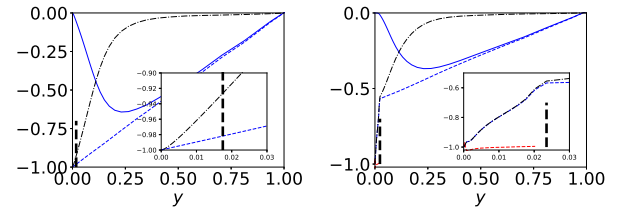
Figure 5: Channel flow. Standard DES (left) and NZ S-DES (right). Shear stresses scaled with u_\tau^2 . Vertical black dashed lines show predicted RANS-LES interface. —: resolved; - - -: viscous + modeled; —: total. - - -: viscous plus modeled in RANS solver (EARSM) in NZ S-DES.
