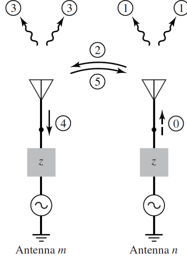
Figure 2.10: Mutual coupling between two antenna elements in the transmitting mode [20].
