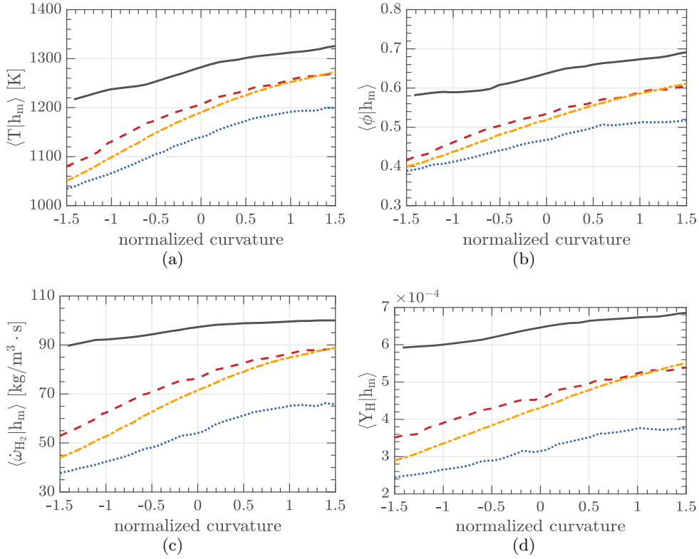
FIGURE 11. Time-averaged dependencies of doubly conditioned (a) temperature \langle T | c = 0.75 | h_m \rangle , (b) equivalence ratio \langle \phi | c = 0.75 | h_m \rangle , (c) fuel consumption rate \langle \dot{\omega}_{H_2} | c = 0.75 | h_m \rangle , and (d) hydrogen mass fraction \langle Y_H | c = 0.75 | h_m \rangle on the normalized local curvature \delta_L h_m , sampled from the entire flame brush (orange dotted-dashed lines), its leading zone characterized by \langle c \rangle(y, t) = 0.1 \pm 0.02 (black solid lines), middle zone ( \langle c \rangle = 0.5 \pm 0.02 , red dashed lines), and trailing zone ( \langle c \rangle = 0.9 \pm 0.02 , blue dotted lines). Case C.
