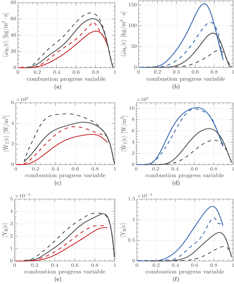
FIGURE 14. Time-averaged dependencies of doubly conditioned (a) and (b) fuel consumption rate \langle \dot{\omega}_{H_2} | c \rangle , (c) and (d) heat release rate \langle \dot{W}_T | c \rangle , and (e) and (f) hydrogen mass fraction \langle Y_H | c \rangle on combustion progress variable, sampled at \langle c \rangle = 0.1 \pm 0.02 (red or blue lines) and 0.9 \pm 0.02 (black lines). Results conditioned to the negative \delta_L h_m = -1 \pm 0.005 or positive \delta_L h_m = 1 \pm 0.005 are shown in dashed or solid lines, respectively. (a), (c), and (e) - case C1/H; (b), (d), and (f) - case C1/H2.
