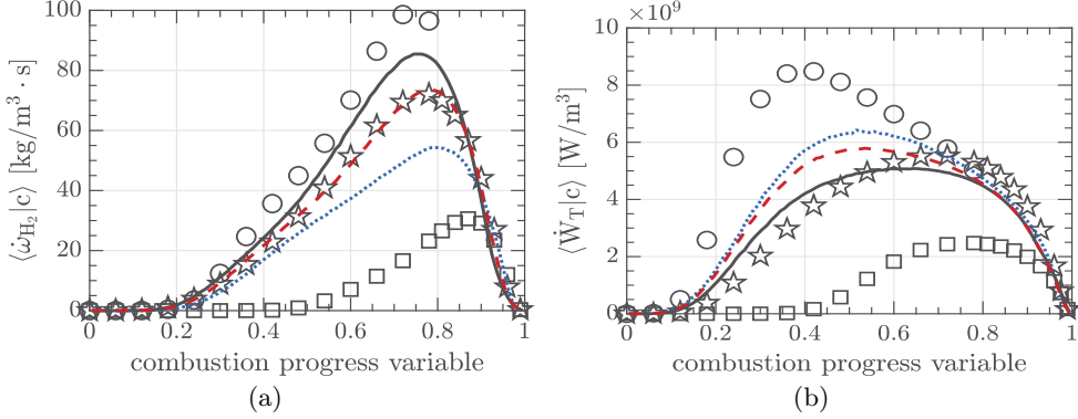
FIGURE 20. Time-averaged dependencies of doubly conditioned (a) fuel consumption rate \langle \dot{\omega}_{H_2} | c \rangle h_m and (b) heat release \langle \dot{W}_T | c \rangle h_m on c , obtained at \delta_L h_m = -0.1 \pm 0.005 (blue dotted lines), 0 \pm 0.005 (red dashed lines), and 1 \pm 0.005 (black solid lines) in case C. Symbols are explained in caption to figure 2.
