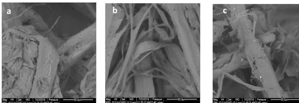
Figure 6. SEM images of (a) unmodified TMP fibres, (b) 95 % TMP + 5 % MgSt and (c) 95 % TMP+ 5 % MoS 2 . Magnification: 800x.
