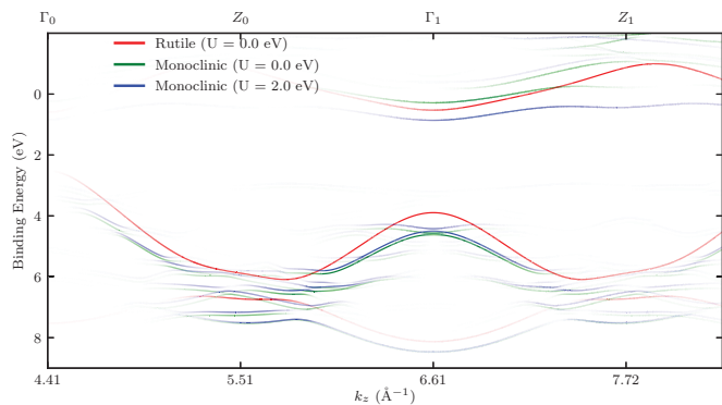
FIG. 9. Band structure plot similar to Fig. 7, but along the \Gamma -Z direction at normal emission (i.e., k_x = 0.00 \text{ \AA}^{-1} ) for the nonmagnetic rutile phase for U = 0.0 \text{ eV} [red, Fig. 4(c)] and the antiferromagnetic monoclinic phase for U = 0.0 \text{ eV} (green) and 2.0 \text{ eV} (blue, Fig. 4(f)).
