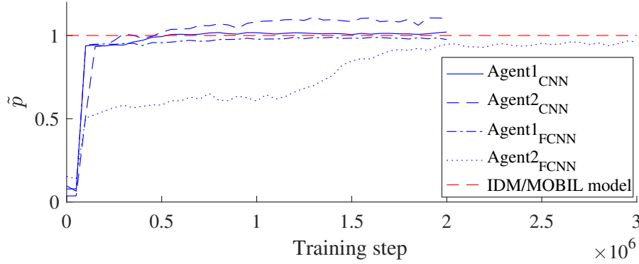
Figure 4.4: Performance index of the different agents during the training process.
