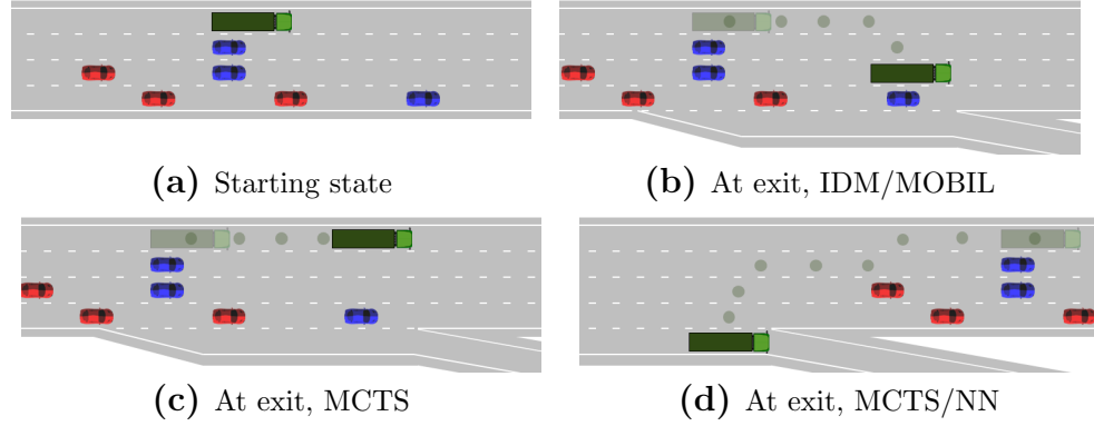
Figure 5.4: Example of when it is necessary to plan relatively far into the future to solve a specific situation. The initial state, 300 m from the exit, is shown in (a), and the state at the exit is shown for the three agents in (b), (c), and (d). The dots show the position of the ego vehicle relative to the other vehicles during the maneuver, i.e., in (b) and (c) the ego vehicle accelerates and overtakes the slower vehicles, whereas in (d), the ego vehicle slows down and ends up behind the same vehicles.
