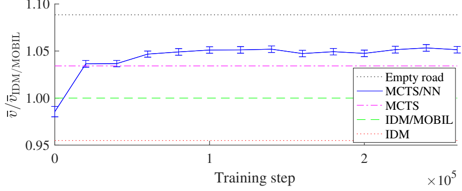
Figure 5.2: Mean speed \bar{v} during the evaluation episodes for the continuous highway driving scenario, normalized with the mean speed of the IDM/MOBIL agent \bar{v}_{IDM/MOBIL} . The error bars indicate the standard error of the mean for the MCTS/NN agent, i.e., \sigma_{\text{sample}}/\sqrt{100} , where \sigma_{\text{sample}} is the standard deviation of the 100 evaluation episodes.
