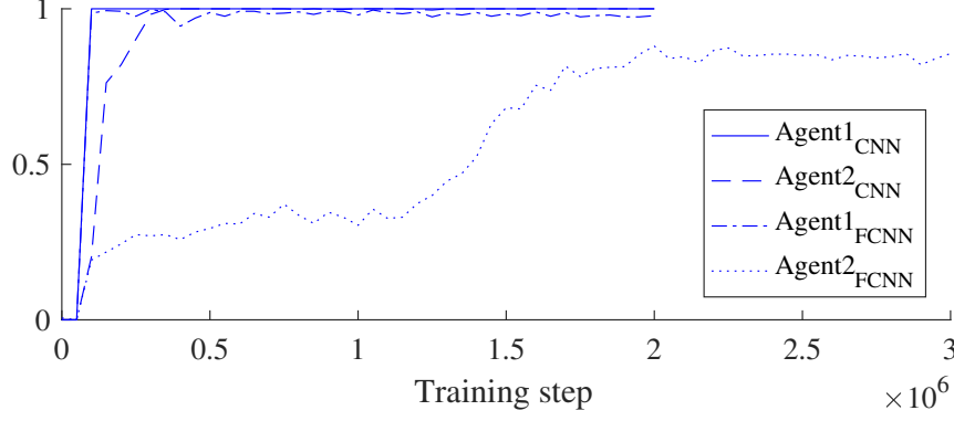
Figure 4.3: Proportion of episodes that are solved without collisions by the different agents during the training process.
