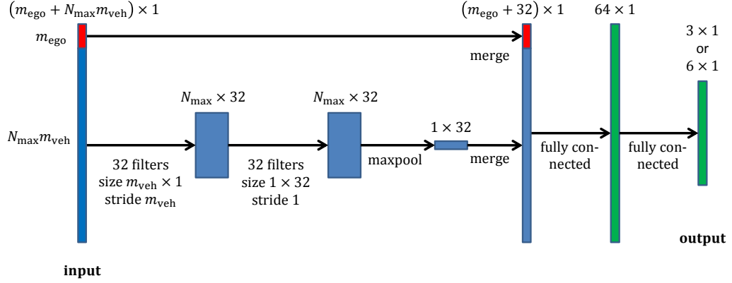
Figure 4.2: The proposed neural network architecture, which uses convolutional layers and max pooling to make the output invariant to permutations of the vehicles in the current traffic situation. The output consists of three and six Q -values for Agent1 and Agent2, respectively, see the main text for further explanations.
