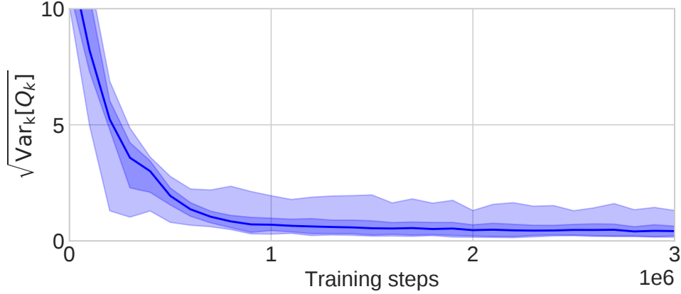
Figure 6.3: Epistemic uncertainty of the chosen actions for the ensemble RPF agent, with parameters \beta = 300 and K = 10 , during testing episodes within the training distribution. The solid line shows the mean, while the shaded regions indicate percentile 10 to 90 and 1 to 99.
