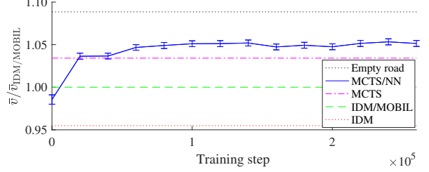
Fig. 4. Mean speed \bar{v} during the evaluation episodes for the continuous highway driving case, normalized with the mean speed of the IDM/MOBIL model \bar{v}_{\text{IDM/MOBIL}} . The error bars indicate the standard error of the mean for the MCTS/NN agent, i.e., \sigma_{\text{sample}}/\sqrt{100} , where \sigma_{\text{sample}} is the standard deviation of the 100 evaluation episodes.
