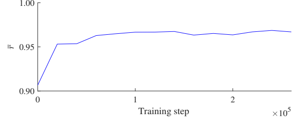
Fig. 3. Average reward per step \bar{r} during the evaluation episodes, as a function of the number of training steps, for the continuous highway driving case.
