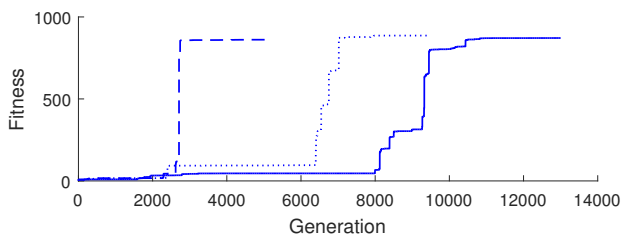
Fig. 6. Fitness variation of the best individual in the population, for three optimization runs with different random seeds.
