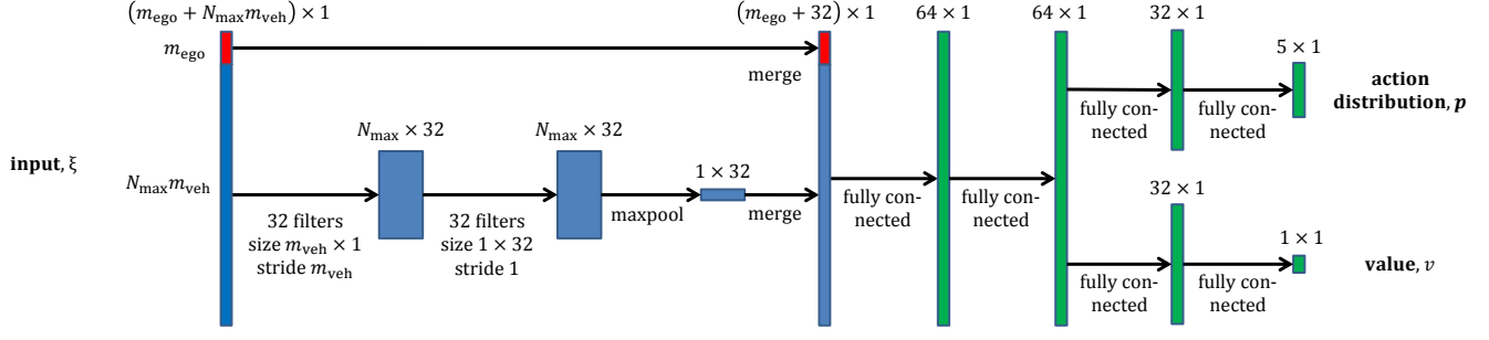
Fig. 2. The figure illustrates the neural network architecture that was used in this study. The convolutional and max pooling layers create a translational invariance between the input from different surrounding vehicles, which makes the ordering and the number of vehicles irrelevant.
