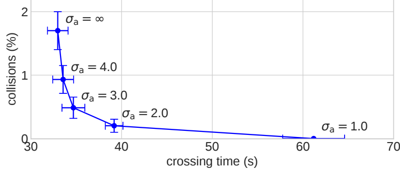
Figure 6.2: Number of collisions and crossing time for the IQN algorithm for different levels of allowed aleatoric uncertainty, which is achieved by varying the parameter \sigma_a .
