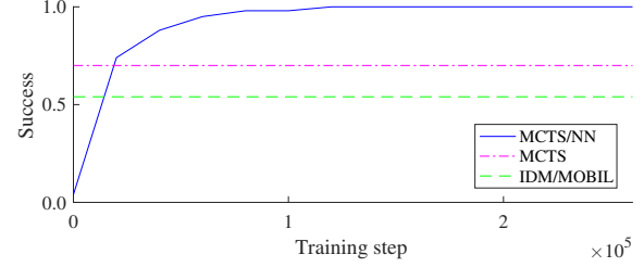
Fig. 7. Proportion of successful evaluation episodes, as a function of training steps, for the highway exit case.
