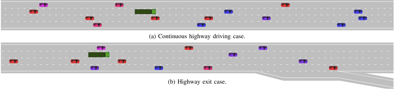
Fig. 1. Examples of the two test cases. (a) shows an initial state for the continuous highway driving case, whereas (b) shows the exit case, when the ego vehicle is approaching the exit on the right side of the road. The ego vehicle is the green truck, whereas the color of the surrounding vehicles represent the aggressiveness level of their corresponding driver models, see Sect. IV-E. Red is an aggressive driver, blue is a timid driver, and the different shades of purple represent levels in between.
