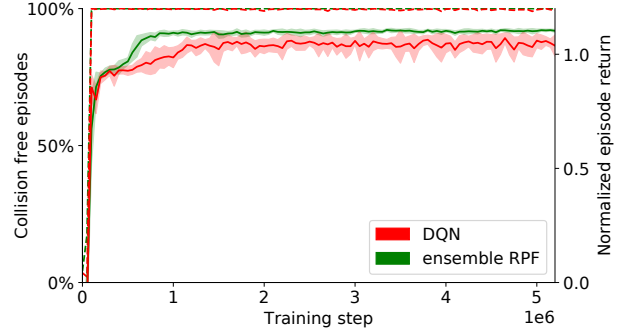
Fig. 3: Proportion of collision free test episodes (dashed), and mean normalized return over training steps for the ensemble RPF and DQN agents (solid). The shaded areas show the standard deviation for 10 random seeds.
