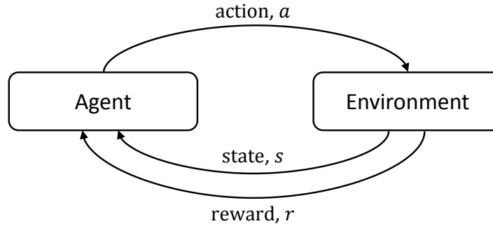
Figure 3.1: In a reinforcement learning problem, an agent learns a policy \pi by interacting with its environment. The agent collects experience by repeatedly taking actions and then observing the resulting state and reward.
