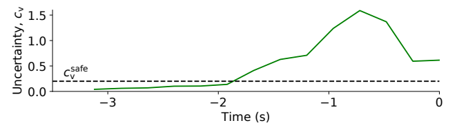
Fig. 6: Uncertainty c_v during the time steps before one of the collisions in the test episodes, within the training distribution. The collision occurs at t = 0 s.
