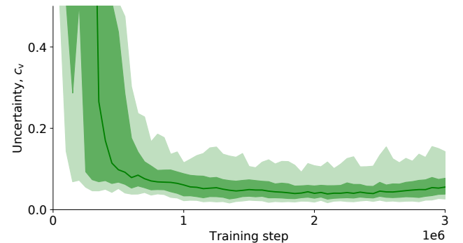
Fig. 5: Mean coefficient of variation c_v for the chosen action during the test episodes. The dark shaded area shows percentiles 10 to 90, and the bright shaded area shows percentiles 1 to 99.
