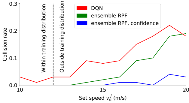
(a) Proportion of collisions.
