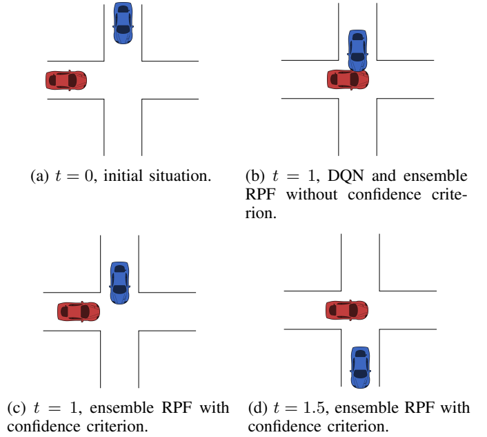
Fig. 8: Example of a situation outside of the training distribution, where there would be a collision if the confidence criterion is not used. The vehicle at the top is here approaching the crossing at 20 m/s.
