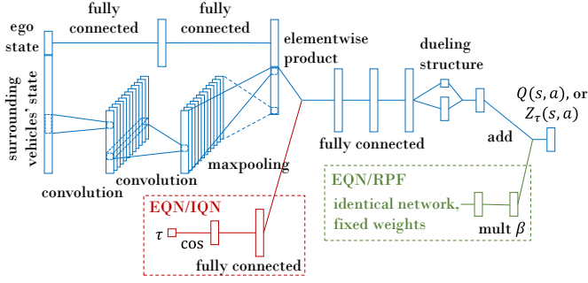
Fig. 2. The neural network architecture that is used for the different agents. The red part is included for the EQN and IQN agents, whereas the green part is included for the EQN and RPF agents.
