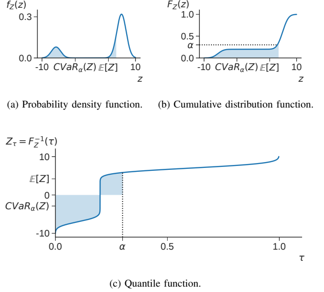
Fig. 1. Illustration of the \text{CVaR}_{\alpha} risk measure. The shaded regions represent quantiles \tau \in [0, \alpha] , here for \alpha = 0.3 .
