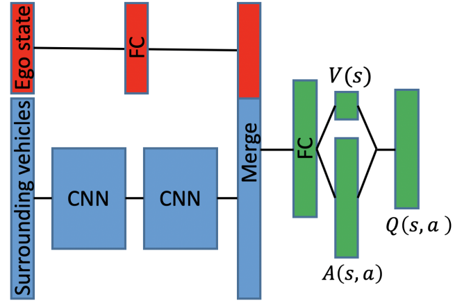
Fig. 3: The neural network architecture that was used in this work.
