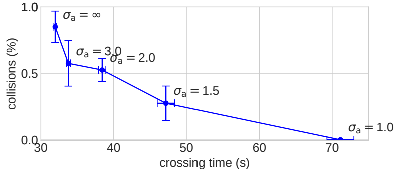
Figure 6.6: Number of collisions and crossing time for the EQN algorithm for different levels of allowed aleatoric uncertainty, which is achieved by varying the parameter \sigma_a .
