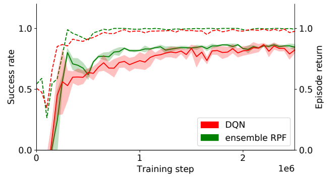
Fig. 4: Proportion of test episodes where the ego vehicle reached its goal (dashed), and episode return (solid), over training steps for the ensemble RPF and DQN methods. The shaded areas show the standard deviation for 5 random seeds.
