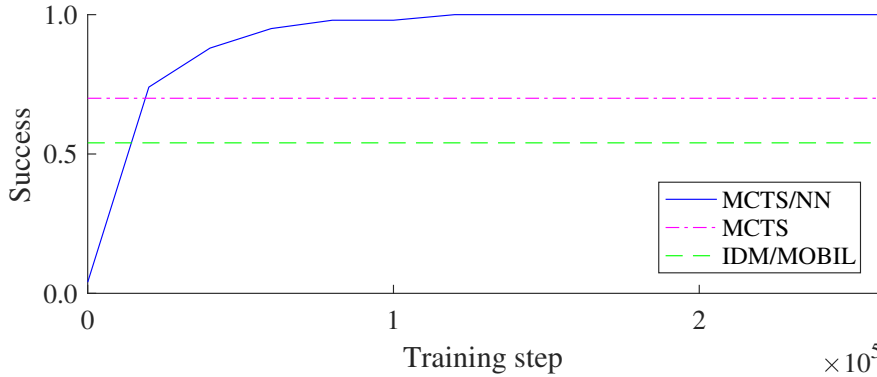
Figure 5.3: Proportion of successful evaluation episodes, as a function of training steps, for the highway exit scenario.
