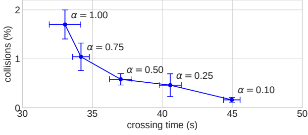
Fig. 5. Number of collisions and crossing time for different levels of risk-sensitive training, which is achieved by varying the CVaR parameter \alpha .
