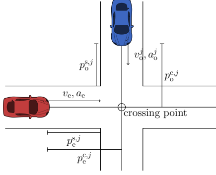
Fig. 2: The state space definitions for a single crossing scenario, where subscript e and o denotes ego and other vehicle, respectively.
