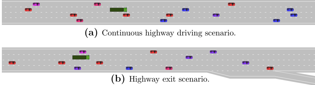
Figure 5.1: The two test scenarios that are used to evaluate the MCTS/NN agent. Panel (a) shows an initial state for the continuous highway driving scenario, whereas panel (b) shows the exit scenario, when the ego vehicle is approaching the exit on the right side of the road. The ego vehicle is the green truck, whereas the colors of the surrounding vehicles represent the aggressiveness level of their corresponding driver models. Red is an aggressive driver, blue is a timid driver, and the different shades of purple represent levels in between. The exact interpretation of aggressiveness level is given in Paper III.
