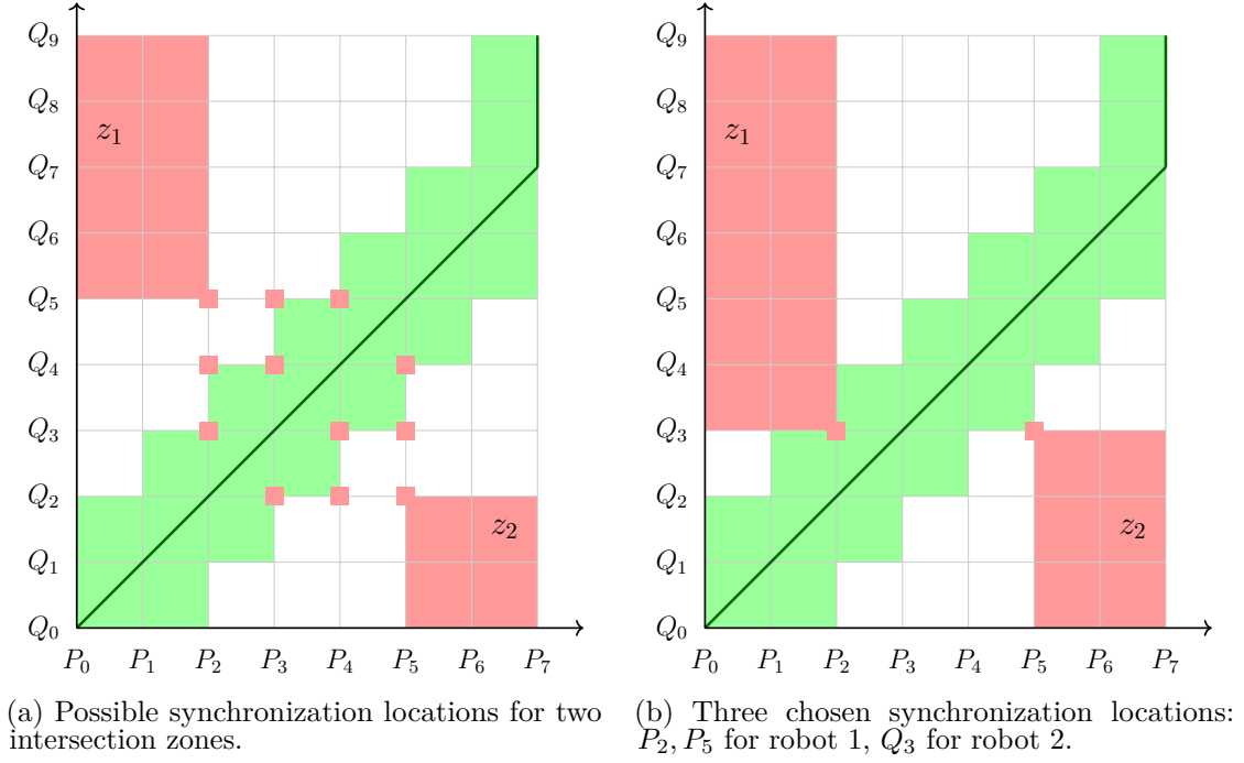
Figure 3.4: Coordination diagram with possible synchronization locations for two intersection zones.
