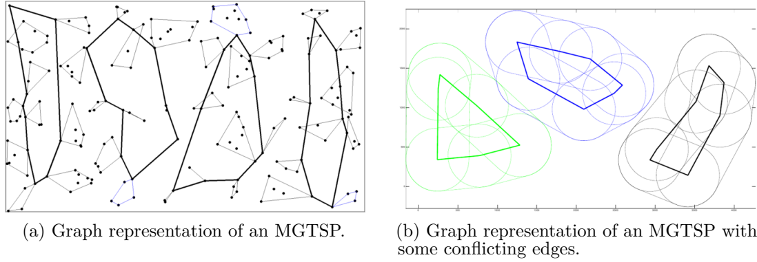
Figure 2.3: MGTSP without and with conflicts.
