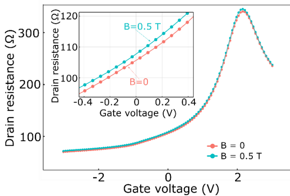
Fig. 1. The drain resistance vs the gate voltage with and without magnetic field. Insert shows the dependences in a narrow range of the gate voltage.
