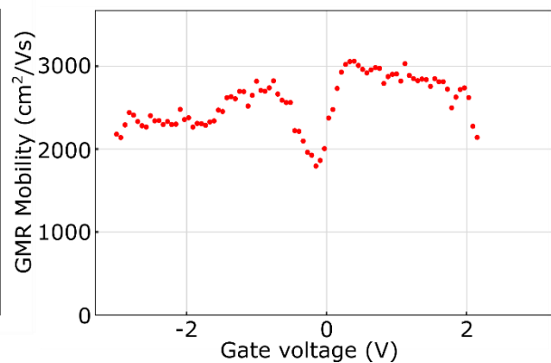
Fig. 2. The GMR mobility vs the gate voltage calculated using data from Fig. 1.
