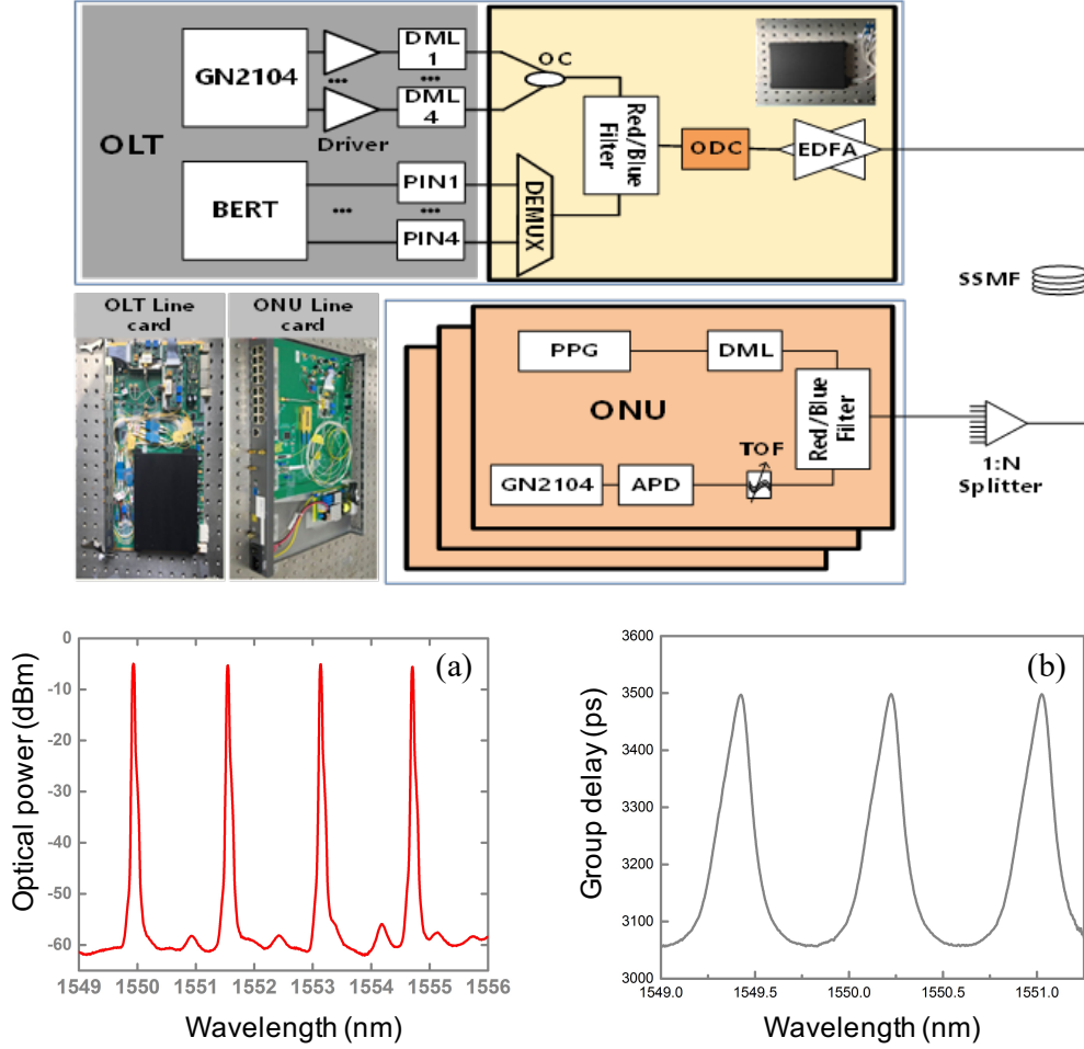
Figure 4.4: Experiment setup for C-band symmetric 4x25 Gb/s PON with 10G optics. Inset: (a) optical spectrum of four channels in downstream; (b) the measured group delay curve of ODC module.
