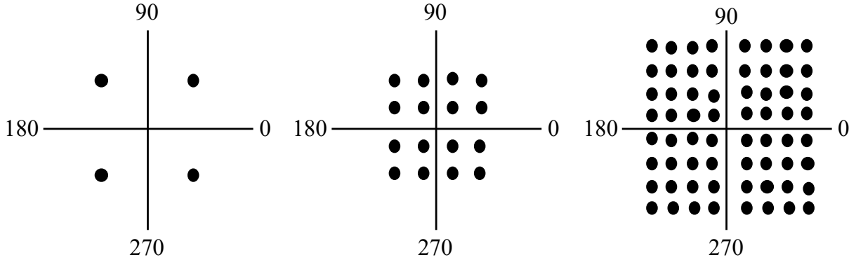
Figure 2.7: Constellation of 4 QAM, 16 QAM and 64 QAM.
