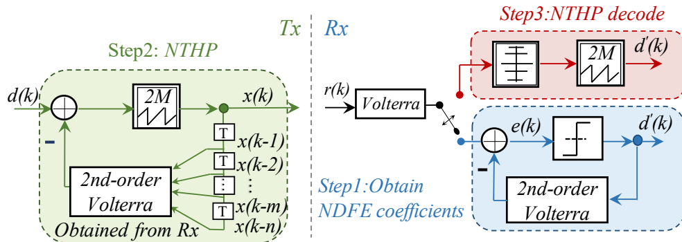
Figure 5.5: Block diagram of NTHP-Volterra equalizer.
