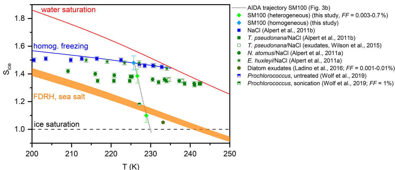
Figure 7. Homogenous and heterogeneous ice nucleation onsets from the AIDA expansion run with the particles generated from the SM100 culture shown in Fig. 3b (light green and blue diamonds) in comparison with data from previous experiments with phytoplankton and marine bacterial species (see Sect. 1.2). The onsets from the immersion freezing measurements with the technique by Alpert et al. (2011a) were evaluated at median freezing temperatures for homogeneous and heterogeneous ice nucleation. The heterogeneous ice nucleation onsets from the AIDA and the various CFDC experiments correspond to different FF values as indicated in the legend and discussed in Sect. 4.1. The S_{\text{ice}} versus T trajectory of the AIDA experiment is shown as the grey line. The other reference lines are the same as shown in Fig. 6.
