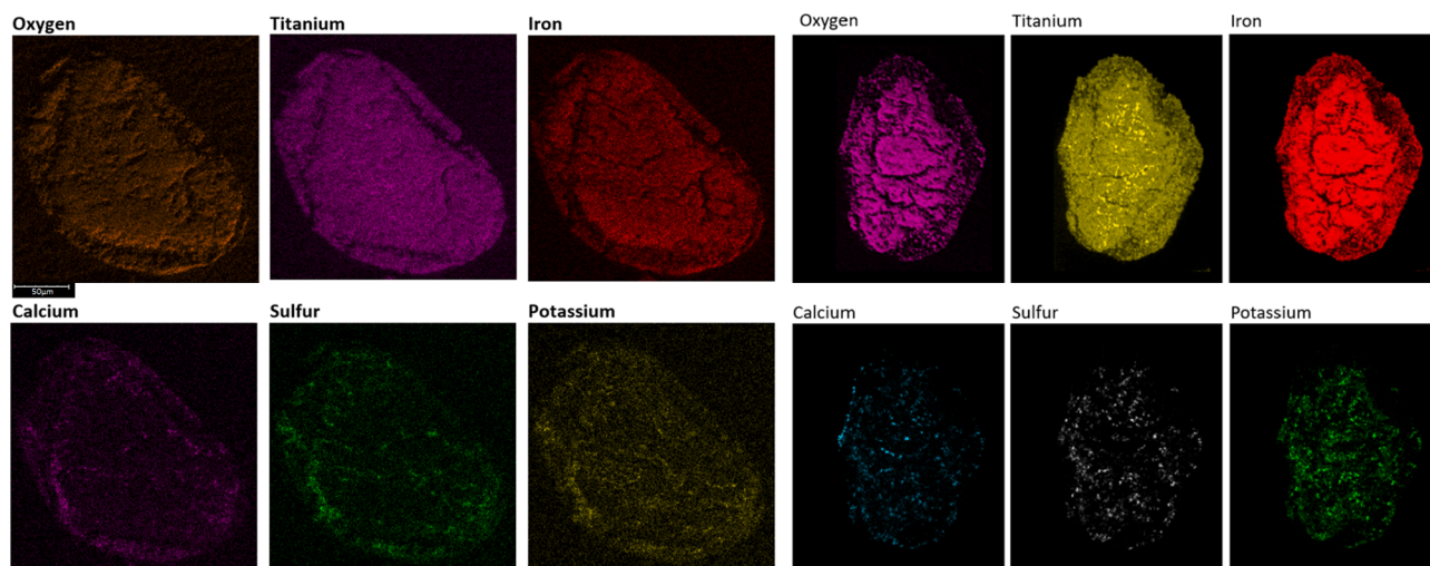
Fig. 8. SEM-EDX intensity maps showing the distributions of O, Ti, Fe, Ca, K and S in the cross-sections of ilmenite particles from Sample I 48H (left) and Sample II 0H (right) after the SO_2 capture experiment in the laboratory-scale reactor.
