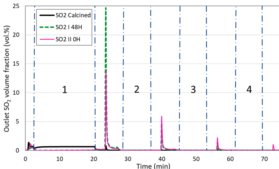
Fig. 5. Levels of SO 2 released from the three selected samples after SO 2 capture. The SO 2 capture at the beginning of the cycle is shown in greater detail in Fig. 4. Zones 1 to 4 represent the oxidizing phases with 5% O 2 in N 2 . Between each numbered area, reduction take place where SO 2 release is visible.
