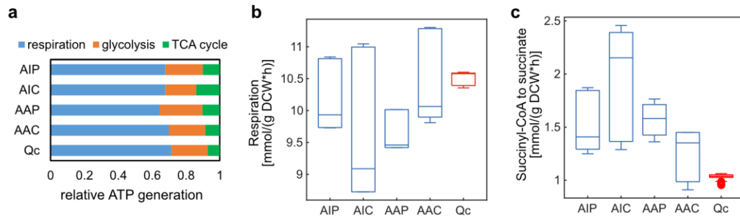
Figure 2-6. Changes in the energy generation pathways. a Relative ATP yield generated from respiration, glycolysis and TCA cycle between strains. b Carriage flux of ATP synthase in the mitochondrion. c Carriage flux of succinyl-CoA to succinate in the TCA cycle.
