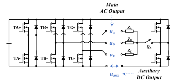
(b) Schematic diagram of the circuit proposed in [13] and evaluated in [14] Fig. 1 Schematic diagrams of the circuits proposed in previous studies which utilize the neutral point of the three-phase load to extract common mode switching harmonics for auxiliary power output
