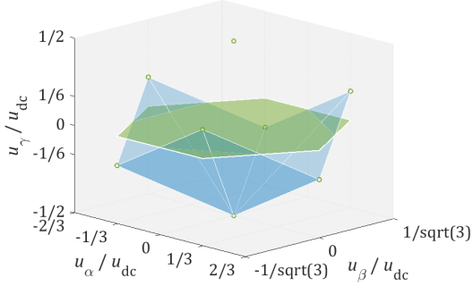
(b) Lower three rhombi &amp; SVM hexagon
