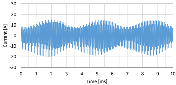
(b) Three-phase load currents & extraction circuit currents
