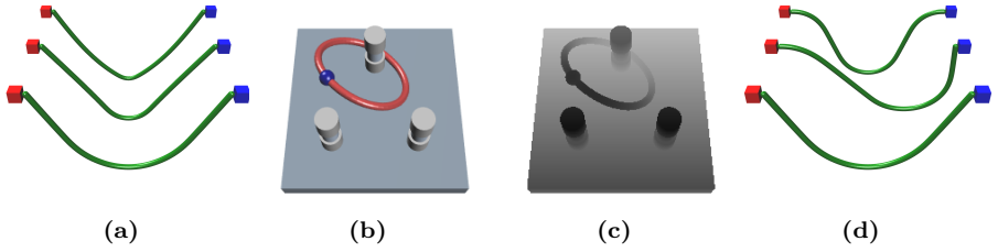
Figure 4: (a) Illustration of the effect of plasticity on the shape of a DLO. All three shapes were generated with identical velocity trajectories, the only difference is the value of the yield point of the DLOs. This property relates to the transition from the elastic to the plastic domain. Examples of visual observations available in ReForm: (b) RGB image (c) Depth image. (d) Illustration of grip compliance changes on the shape of DLOs with identical mechanical properties, and identical trajectories.
