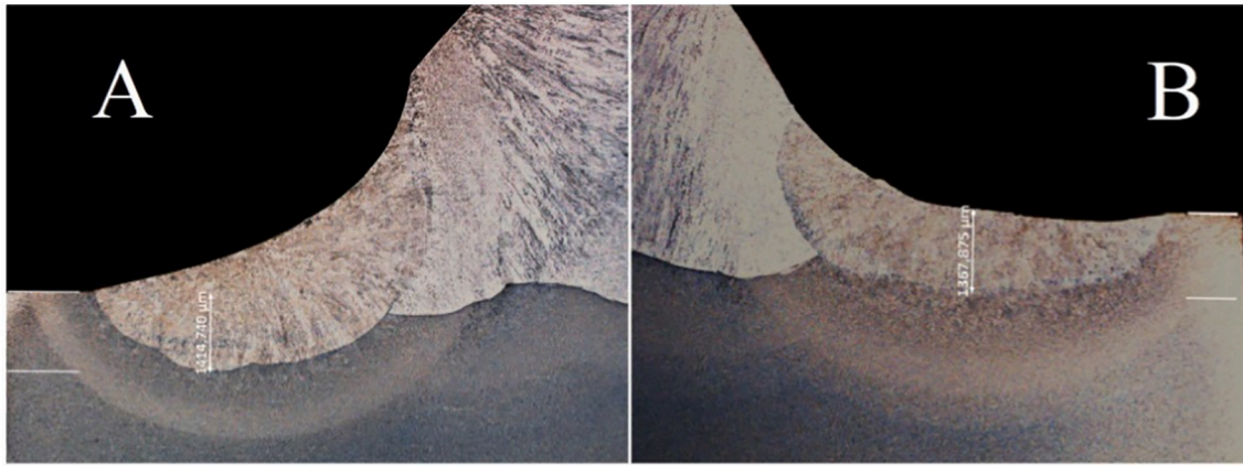
Fig. 24. Fusion depth when the TIG electrode is placed A: Directly at the weld toe B: according to the IIW recommendations [5].
