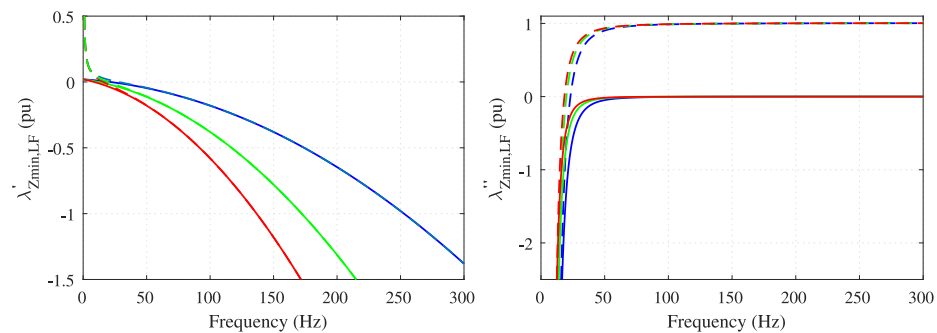
Figure 12. Frequency characteristic of \lambda'_{Z_{min,LF}} (left) and \lambda''_{Z_{min,LF}} (right) with R_v = 0.02 pu and L_v = 0.2 pu (blue), L_v = 0.4 pu (green), and L_v = 0.6 pu (red); solid curves represent the case of considering only the virtual-impedance dependent term (exp-1) from Z'_{conv,LF} and Z''_{conv,LF} .
