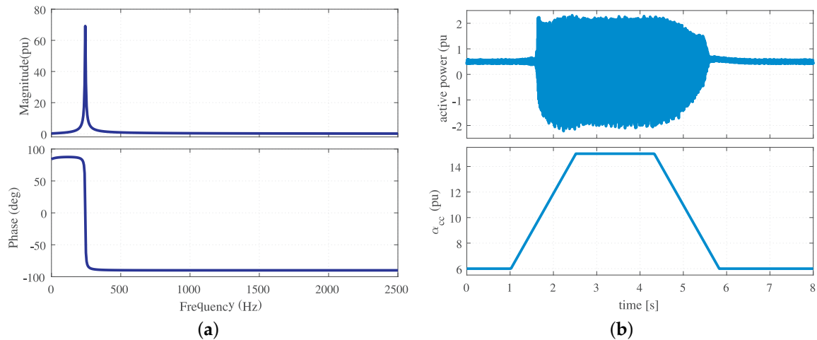
Figure 9. (a) Frequency response of the connection-grid impedance, Z_{\text{grid}} ; (b) active-power output of the converter with a resonance grid connection and R_v = R_f , L_v = L_f during a change in the current-controller bandwidth, \alpha_{cc} .
