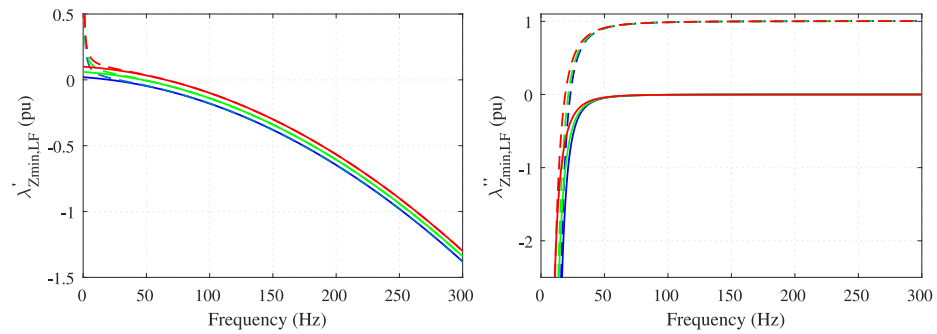
Figure 11. Frequency characteristic of \lambda'_{Z_{min,LF}} (left) and \lambda''_{Z_{min,LF}} (right) with L_v = 0.2 pu and R_v = 0.02 pu (blue), R_v = 0.06 pu (green), and R_v = 0.10 pu (red); solid curves represent the case of considering only the virtual-impedance dependent term (exp-1) from Z'_{conv,LF} and Z''_{conv,LF} .
