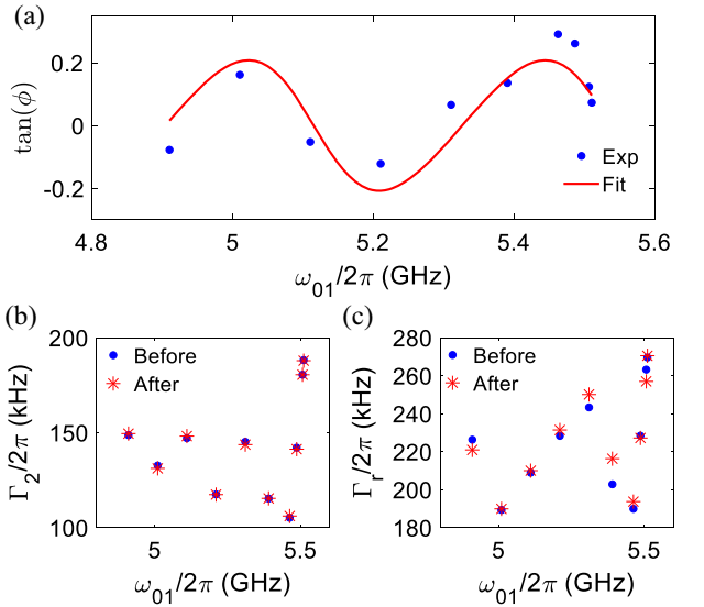
Fig. 9 Compensating the Fano-shape reflection coefficient. a The phase \phi in Eq. (4) vs. different qubit frequencies. Blue dots are the data with the solid curve as a fit. b , c The comparison of \Gamma_2 and \Gamma_r before and after compensating the impedance mismatch.
