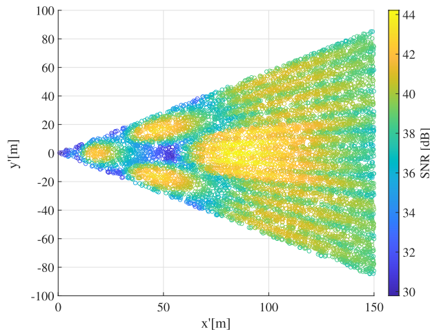
FIGURE 7. Heat map plot of the achievable SNR for SISO mode communications for a single-sector scenario.
