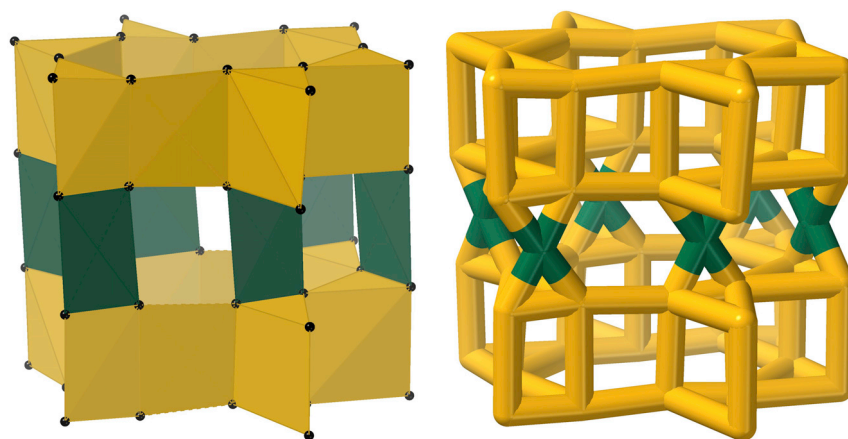
Figure 11. The network in [\text{Ce}_3(\text{btec})(\text{Hbtec})(\text{OAc})(\text{HCO}_2)] : CTH-15
