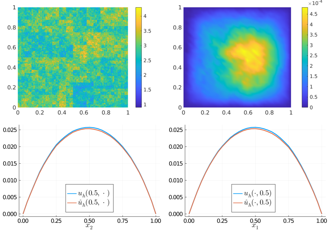
FIGURE 4.2. Results of Experiment 1: unstructured multiscale coefficient sampled from \mathfrak{A}_{ms} (top left), |u_h(x) - \hat{u}_h(x)| (top right) and comparison of u_h vs. \hat{u}_h along the cross sections x_1 = 0.5 (bottom left) and x_2 = 0.5 (bottom right).
