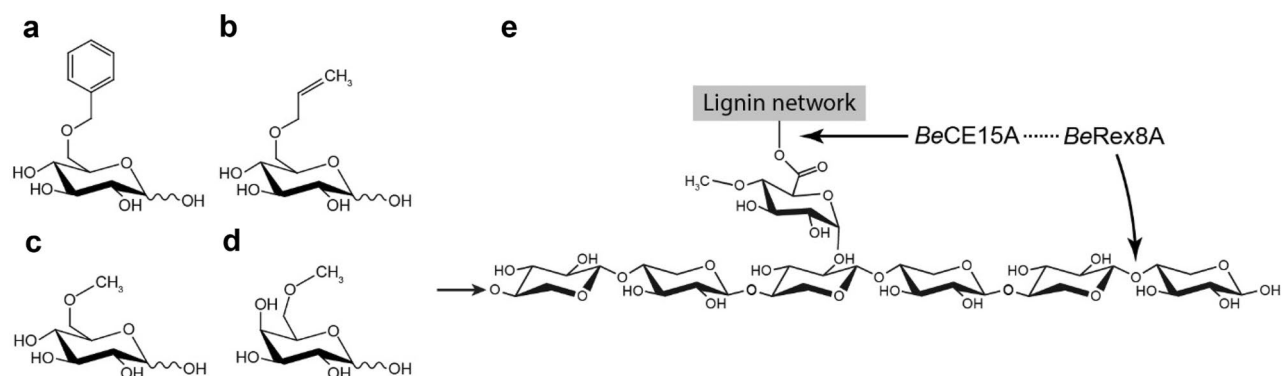
Figure 3. Substrates used to assay glucuronoyl esterase activity of BeCE15A : (a) benzyl glucuronate, (b) allyl glucuronate, (c) methyl glucuronate, and (d) methyl galacturonate. (e) The suggested target of the full-length BeCE15A -Rex8A enzyme, consists of a xylooligosaccharide (or longer xylan chain as indicated by the small arrow) decorated with GlcA, which is further ester-linked to lignin or lignin fragments.
