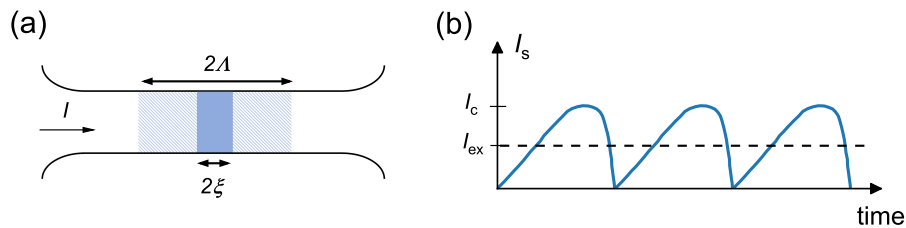
Figure 8.3: (a) Illustration of the PSC model in a nanowire. (b) Oscillations of the superconducting part of the current I_s in the PSC. I_{\text{ex}} is the average I_s through the PSC (dashed line). See the text for a description. Adapted from Ref. [153].
