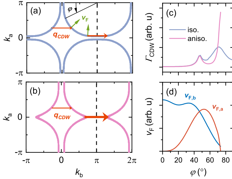
Figure 6.6: Uniaxial CDW scattering on (a) isotropic and (b) anisotropic Fermi surface. The red arrows shows the CDW scattering vector where the size is proportional to the scattering rate. The green arrows show the direction of the Fermi velocity at the CDW scattering points. (c) Angular dependence of the CDW scattering rate in for the isotropic Fermi surface in (a) and the anisotropic Fermi surface in (b). (d) Fermi velocity versus the angle \phi defined in (a) for the anisotropic Fermi surface in (b).
