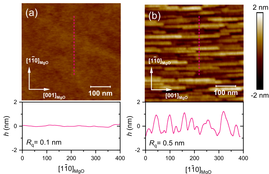
Figure 3.4: AFM images of the surface of a MgO(110) substrate before and after 5 hours of thermal annealing at T = 790^\circ\text{C} . The pink dashed lines are the cuts for the line profiles of the AFM images below.
