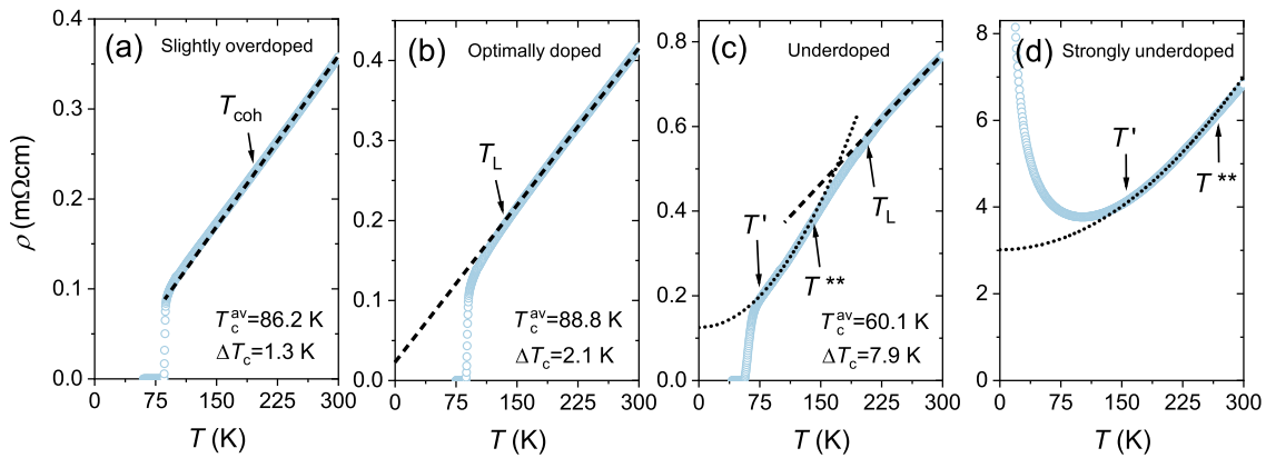
Figure 3.14: Typical \rho(T) of YBCO at different doping levels (a) Slightly overdoped, (b) Optimally doped, (c) Underdoped, (d) Strongly underdoped/undoped. The different characteristic temperatures that can be extracted from the shape of the \rho(T) are pointed out. See the text for a description of each characteristic temperature.
