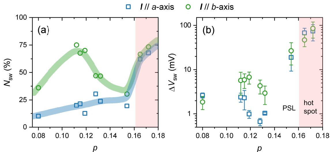
Figure 8.5: Doping dependence of the hysteric voltage switching in 12nm thick YBCO nanowires. (a) Fraction of nanowires ( N_{sw} ) that show hysteric voltage switching. Each point corresponds to \approx 25 nanowires of varying width. (b) Average magnitude of the hysteric voltage switches ( \Delta V_{sw} ). The error bars correspond to \pm one standard deviation. There is less statistics for the wires along the a -axis since a smaller fraction showed switching behavior.
