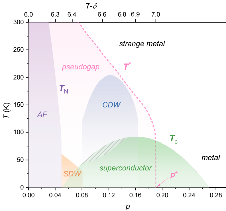
Figure 2.3: Phase diagram of YBCO. On the bottom x-axis, p is the number of holes per planar Cu; on the top x-axis 7-\delta is the oxygen content. From left to right: antiferromagnetic order (AF) below the Néel temperature T_N , spin density waves (SDW), charge density wave (CDW), superconductivity below the critical temperature T_c , pseudogap below T^* (that terminates at p^* \approx 0.19 ), strange metal above T^* and conventional metal at high doping and low temperature.
