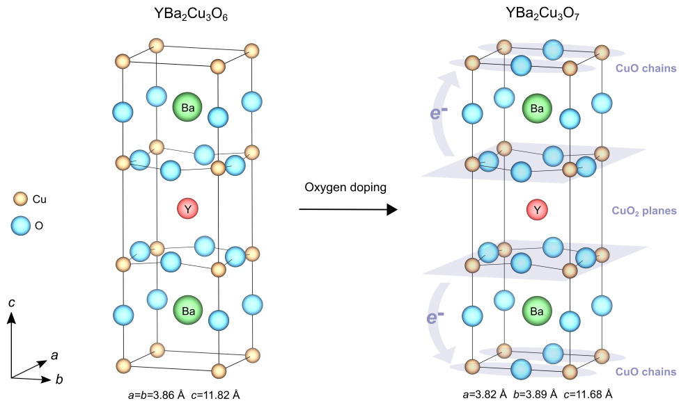
Figure 2.2: Illustration of the crystal structure and hole doping mechanism of YBCO. The left picture shows the tetragonal undoped parent compound \text{YBa}_2\text{Cu}_3\text{O}_6 and the right picture the orthorhombic fully oxygenated \text{YBa}_2\text{Cu}_3\text{O}_7 . The \text{CuO} chains and the \text{CuO}_2 planes are highlighted in the right picture together with the hole doping mechanism [43].
