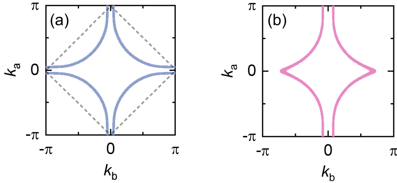
Figure 6.3: Example of Fermi surface modification that is compatible with the higher resistivity anisotropy in the 10 nm thick film on MgO. (a) Typical Fermi surface of the cuprates ( t_a = t_b ) (b) t_b > t_a . The effects of the CuO chains and bi-layer splitting is neglected.
