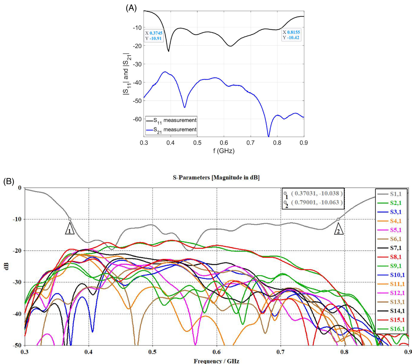
FIGURE 4 (A) Measured return loss and the mutual coupling between the two elements shown in Figure 2A. (B) Simulated return loss and the cross-talk between the 16 elements in the array configuration of Figure 3B [Color figure can be viewed at wileyonlinelibrary.com ]
