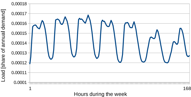
(b) Weekly variations of the electricity demand in region in Sweden.
