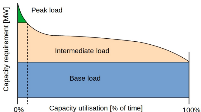
Figure 2.3: A load duration curve to illustrate how base, intermediate and peak load are used in the electricity system. The curve corresponds to the annual load, sorted according to the size of the load.
