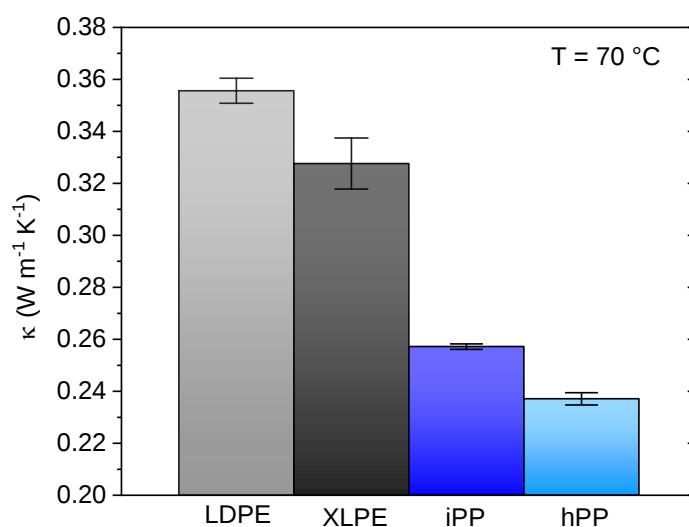
Figure 12. Thermal conductivity \kappa of LDPE (grey), XLPE (black), iPP (blue), and hPP (sky blue), at 70^\circ\text{C} ; error bars are based on the standard deviation calculated from 5 measurements of each sample.
