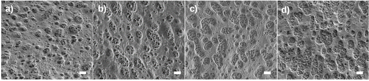
Figure 25. SEM images of cryofractured, etched and sputtered surfaces of 24:76 iPP:(SEBS B :LDPE) ternary blends with SEBS B content: (a) 5 wt%, (b) 10 wt% (c) 20 wt% and (d) 30 wt% (scale bar = 2 μm).
