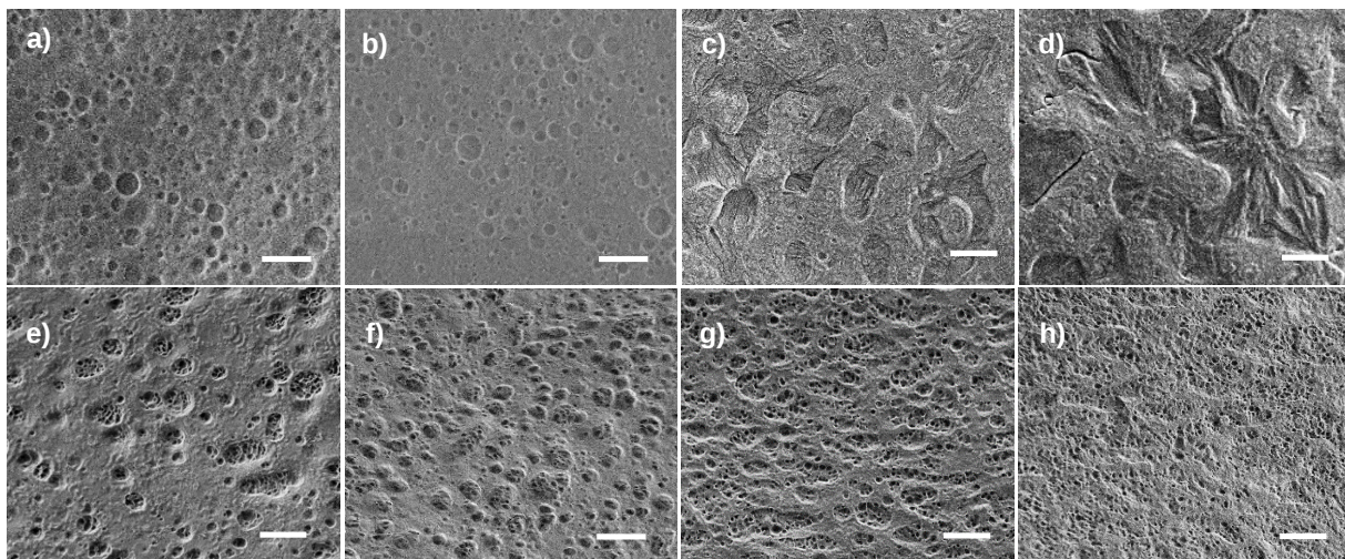
Figure 23. SEM images of cryofractured, etched and sputtered surfaces of iPP:LDPE binary blends with iPP:LDPE ratios of: (a) 20:80, (b) 25:75 (c) 40:60 and (d) 60:40, and the 5:95 SEBS B :(iPP:LDPE) ternary blends with iPP:LDPE ratios of: (e) 20:80, (f) 25:75 (g) 40:60 and (h) 60:40 (scale bar = 5 μm).
