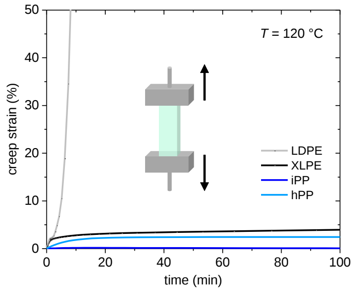
Figure 10. Creep strain at a constant stress of 1 kPa (equivalent to sample weight) at 120 °C as a function of time, of LDPE (grey), XLPE (black), iPP (blue), and hPP (sky blue); inset: schematic of the creep measurement indicating the direction of the applied stress.
