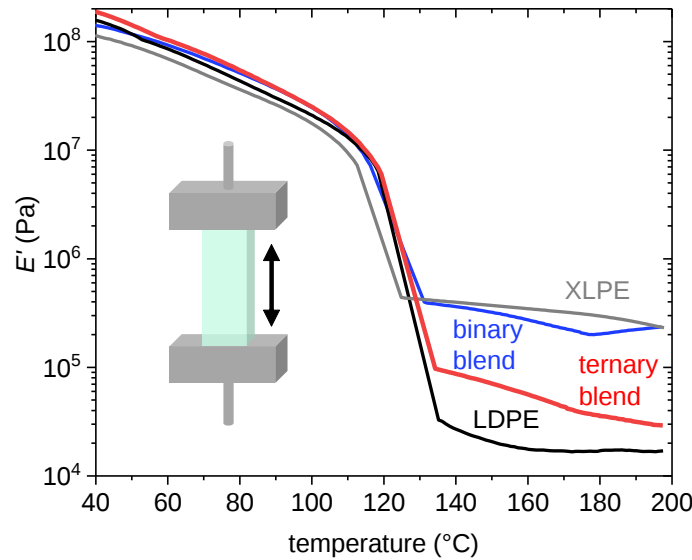
Figure 15. Storage modulus E' measured with DMA as a function of temperature of the 4:1 p(E-stat-GMA):iPP-graft-MA binary blend compounded at 170 °C for 5 minutes (blue), the 24:6:70 p(E-stat-GMA):iPP-graft-MA:LDPE ternary blend compounded at 170 °C for 10 minutes (red), as well as LDPE (black) and XLPE, i.e. LDPE crosslinked with 1 wt% dicumyl peroxide (DCP) at 200 °C (grey); inset: schematic of the oscillatory DMA measurement indicating the direction of the applied stress.
