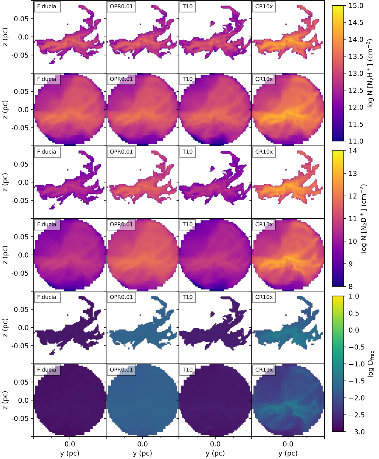
Figure 5. The projections of N_2H^+ , N_2D^+ , and D_{\text{frac}}^{N_2H^+} along the x -axis at 0.8 t_{\text{ff}} . These quantities are plotted in two cases (with density threshold and without density threshold) to display the general concentration properties (see text). The ambient gas is subtracted by limiting the volume inside 0.1 pc sphere. Each column represents a different model (left to right): fiducial; OPR0.01; T10; CR10x, with parameters of these models listed in Table 1. The remaining models are plotted in Figure 6 and 8
