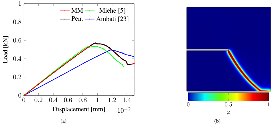
Figure 5: Figure (a) presents the load-displacement curves for the single edge notched specimen under shear. Here, MM and Pen. refer to the Method of Multipliers and the Penalisation method respectively. Figure (b) shows the distribution of the phase-field variable at the final step of the analysis.
