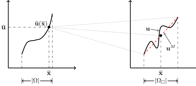
Figure 3.1: Figures showing the smooth solution field \bar{\mathbf{u}} on the macro-scale domain \Omega (left), and the rapidly oscillating solution field \mathbf{u} on the RVE domain \Omega_\square (right). The linear macro-scale contribution \mathbf{u}^M from \bar{\mathbf{u}} is denoted by the dashed red line in the right sub-figure.
