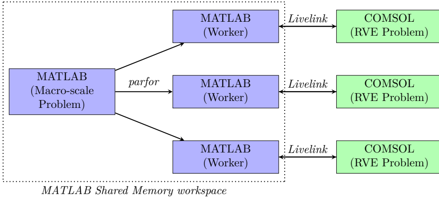
Figure 1.2: An illustration of the MATLAB-COMSOL interaction for a multi-scale \text{FE}^2 problem.
