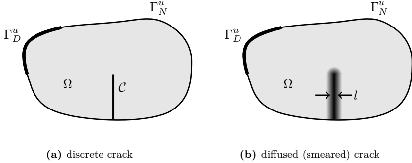
Figure 2.1: A solid \Omega \in \mathbb{R}^2 embedded with (a). discrete crack \mathcal{C} and (b). diffused (smeared) crack, with Dirichlet and Neumann boundaries indicated as \Gamma_D^u and \Gamma_N^u respectively. Figure reproduced from [72].
