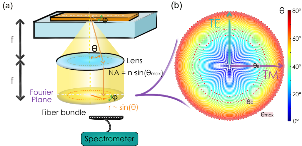
FIGURE 5.1: Fourier spectroscopy concept. (a) Schema of the experimental setup for angle resolution. Collimated light incident to the lens is focused in the sample, such that the incident light to the sample comes at all the angles up to \theta_{max} = \arcsin NA/n . The reflected signal is collected with the same lens. The Back Focal Plane (BFP) of the lens is then imaged and the spectra at different radii are collected simultaneously via a fiber bundle with a spectrometer. (b) Angular distribution of the BFP for an oil immersion objective with NA=1.49 . Brewster, \theta_B , and critical, \theta_C , angles are marked in red dashed lines. The lines for TE and TM mark the locations to measure those polarizations.
