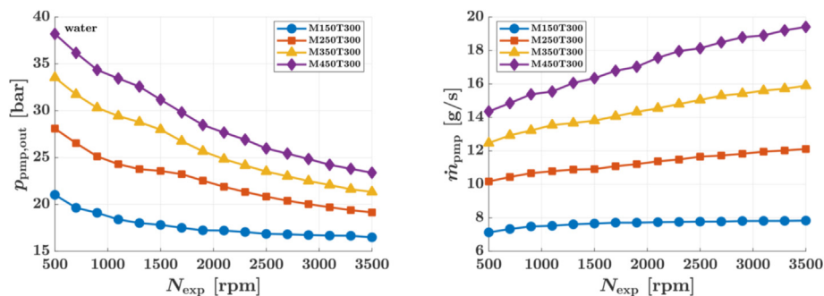
Fig. 19. Pump outlet pressure (left) and mass flow rate (right) for water as functions of the expander speed at different engine operating points.
