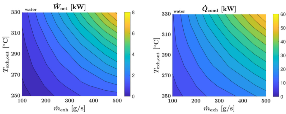
Fig. 21. Net shaft power (left) and condenser heat transfer rate (right) for water as a function of the exhaust mass flow and temperature. The values at the edges were linearly extrapolated.
