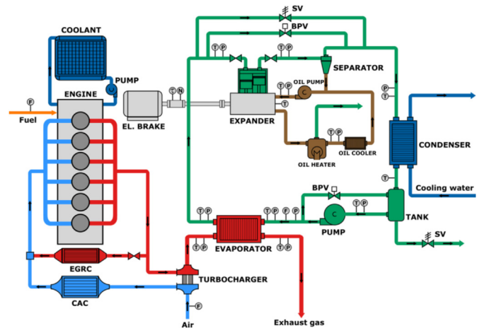
Fig. 2. Schematic depiction of the experimental setup.
