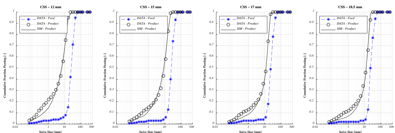
Figure 11. Crusher calibration result to the belt-cut experimental data in the cumulative domain.
